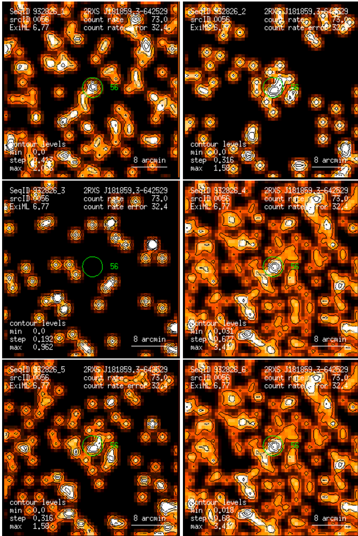
Figure 56: RASS 932826: detection 0056: band rate images, Gaussian filter: (1) PSPC channels 11 – 41, (2) 52 – 90, (3) 91 – 201, (4) 11 – 235, (5) 52 – 201, (6) 11 – 201. Broad band rates in counts/ks. Band rate contour levels in counts/ks/arcmin 2 .
