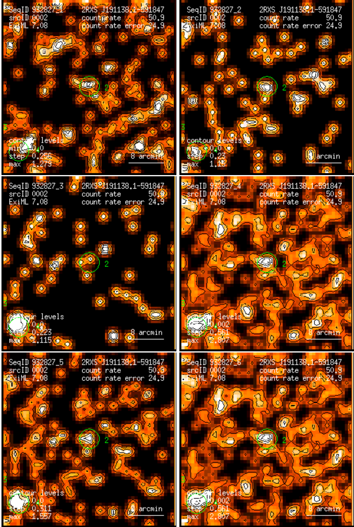
Figure 2: RASS 932827: detection 0002: band rate images, Gaussian filter: (1) PSPC channels 11 – 41, (2) 52 – 90, (3) 91 – 201, (4) 11 – 235, (5) 52 – 201, (6) 11 – 201. Broad band rates in counts/ks. Band rate contour levels in counts/ks/arcmin 2 .
