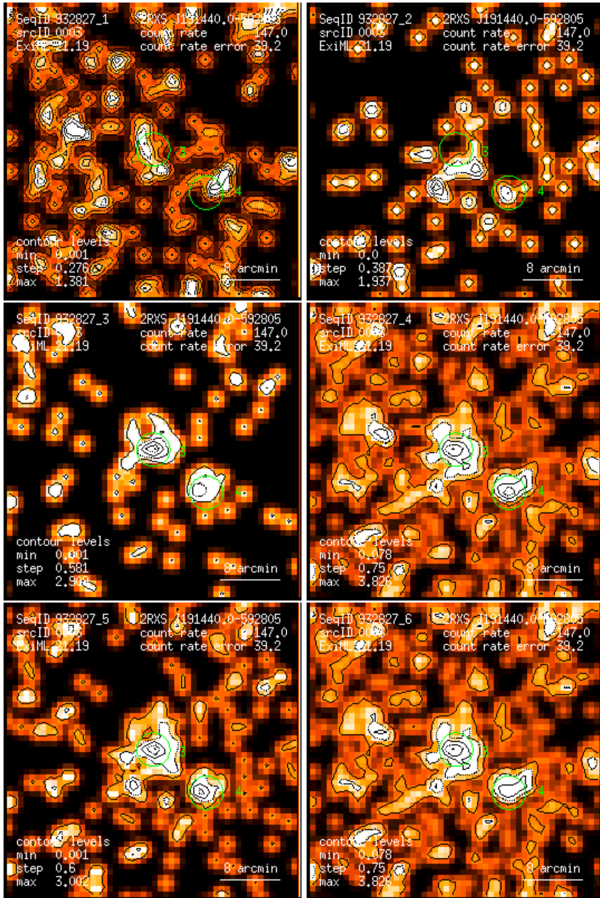
Figure 3: RASS 932827: detection 0003: band rate images, Gaussian filter: (1) PSPC channels 11 – 41, (2) 52 – 90, (3) 91 – 201, (4) 11 – 235, (5) 52 – 201, (6) 11 – 201. Broad band rates in counts/ks. Band rate contour levels in counts/ks/arcmin 2 .
