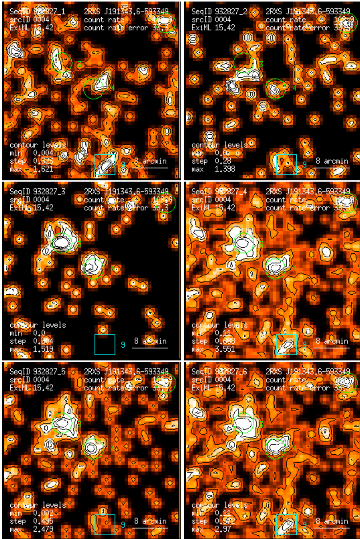
Figure 4: RASS 932827: detection 0004: band rate images, Gaussian filter: (1) PSPC channels 11 – 41, (2) 52 – 90, (3) 91 – 201, (4) 11 – 235, (5) 52 – 201, (6) 11 – 201. Broad band rates in counts/ks. Band rate contour levels in counts/ks/arcmin 2 .
