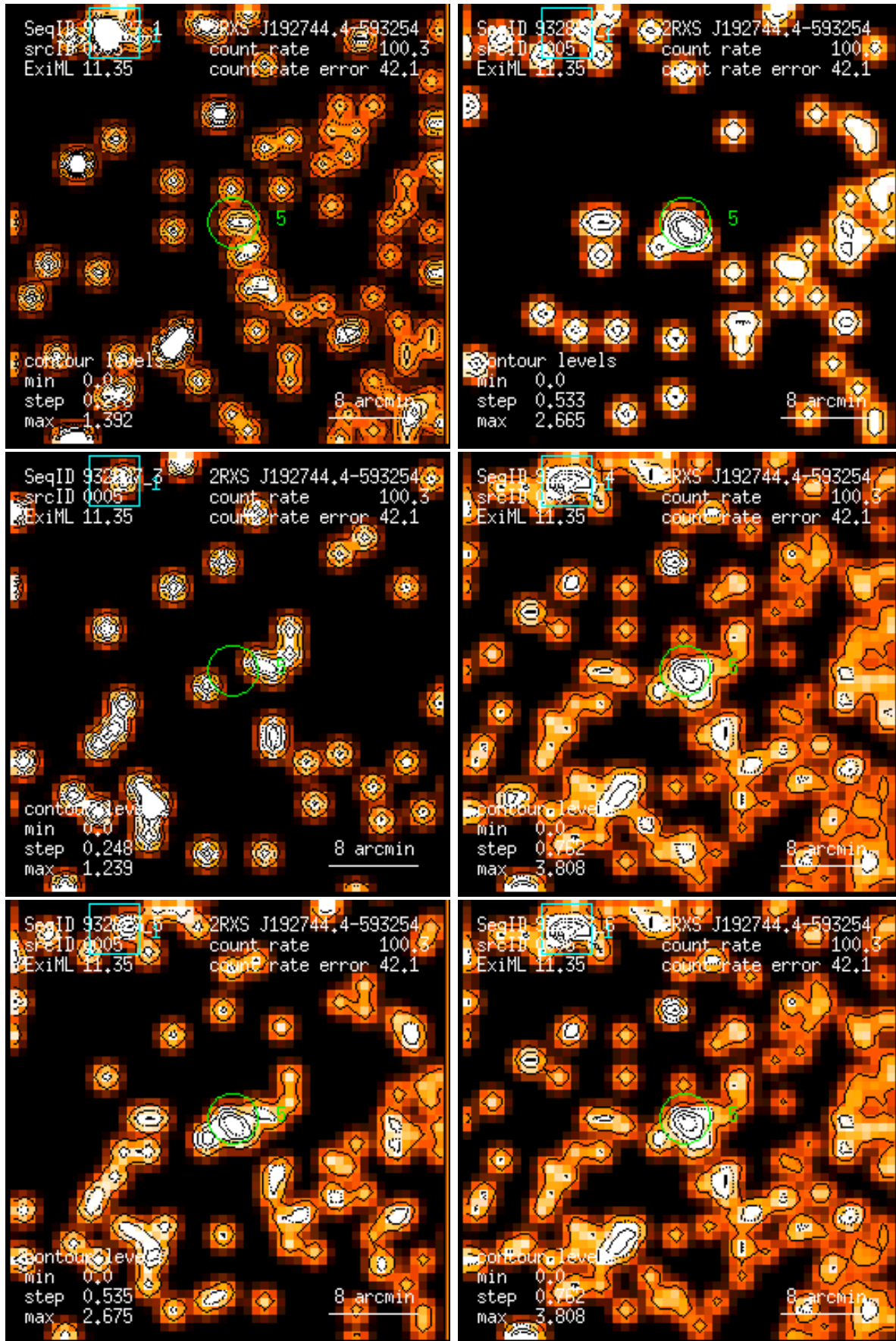
Figure 5: RASS 932827: detection 0005: band rate images, Gaussian filter: (1) PSPC channels 11 – 41, (2) 52 – 90, (3) 91 – 201, (4) 11 – 235, (5) 52 – 201, (6) 11 – 201. Broad band rates in counts/ks. Band rate contour levels in counts/ks/arcmin 2 .
