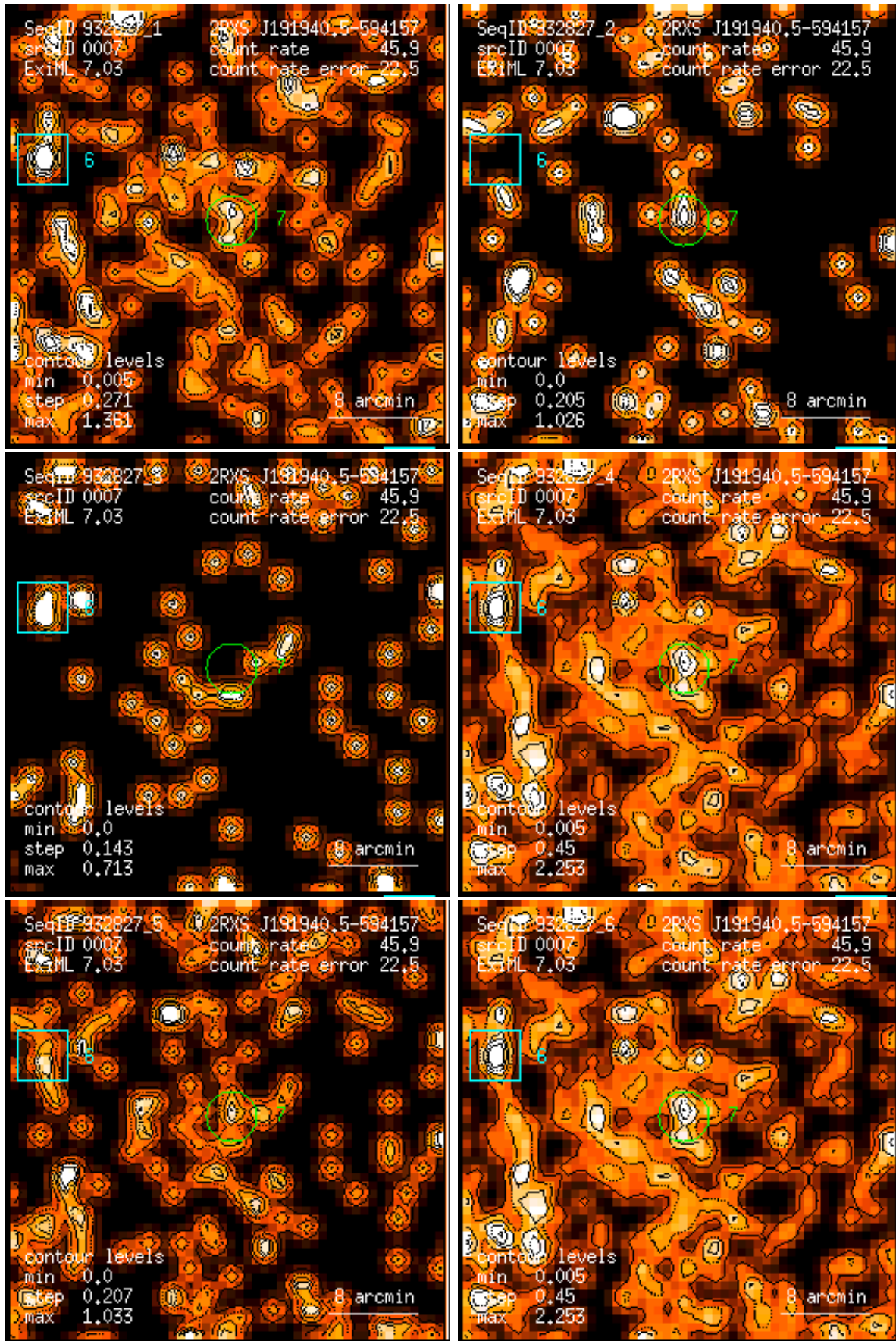
Figure 7: RASS 932827: detection 0007: band rate images, Gaussian filter: (1) PSPC channels 11 – 41, (2) 52 – 90, (3) 91 – 201, (4) 11 – 235, (5) 52 – 201, (6) 11 – 201. Broad band rates in counts/ks. Band rate contour levels in counts/ks/arcmin 2 .
