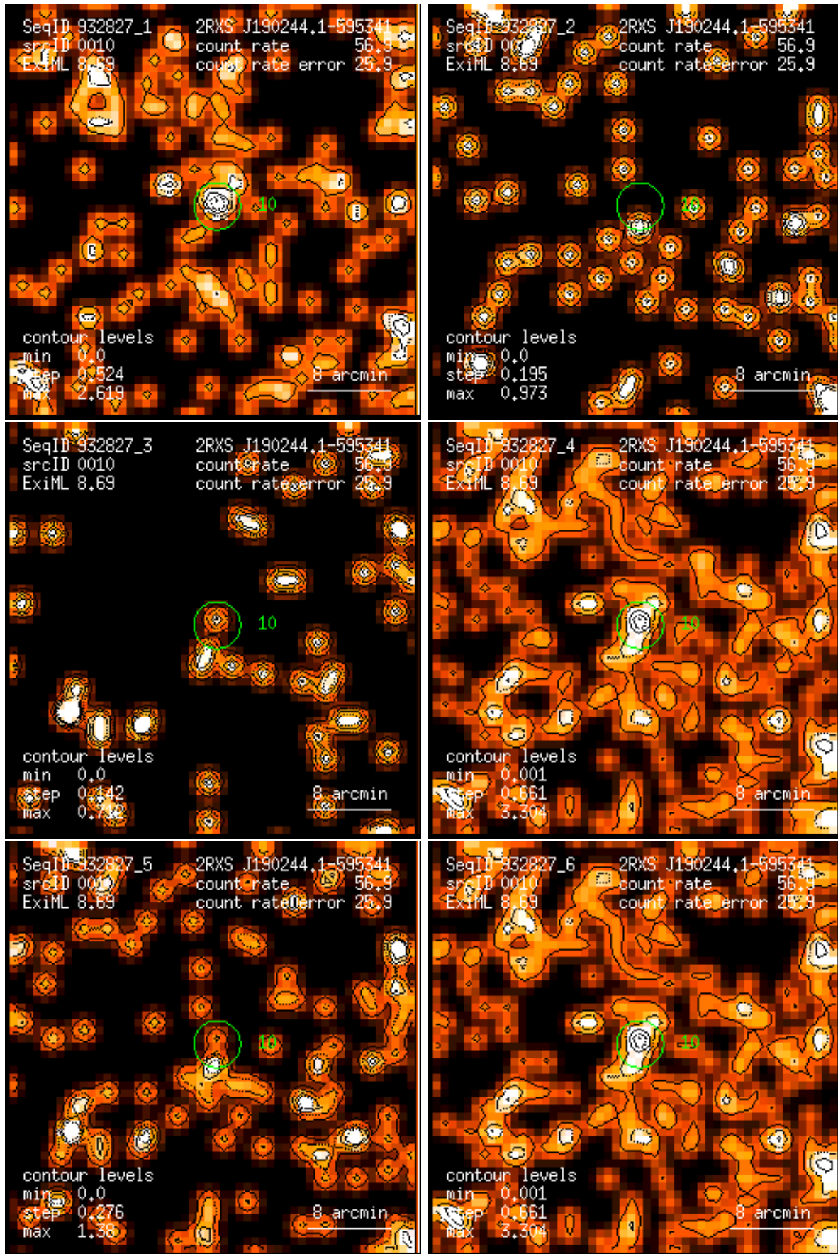
Figure 10: RASS 932827: detection 0010: band rate images, Gaussian filter: (1) PSPC channels 11 – 41, (2) 52 – 90, (3) 91 – 201, (4) 11 – 235, (5) 52 – 201, (6) 11 – 201. Broad band rates in counts/ks. Band rate contour levels in counts/ks/arcmin 2 .
