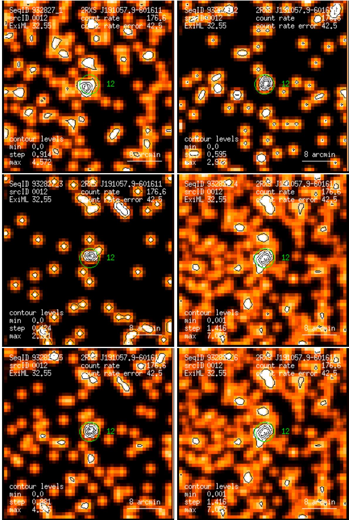
Figure 12: RASS 932827: detection 0012: band rate images, Gaussian filter: (1) PSPC channels 11 – 41, (2) 52 – 90, (3) 91 – 201, (4) 11 – 235, (5) 52 – 201, (6) 11 – 201. Broad band rates in counts/ks. Band rate contour levels in counts/ks/arcmin 2 .
