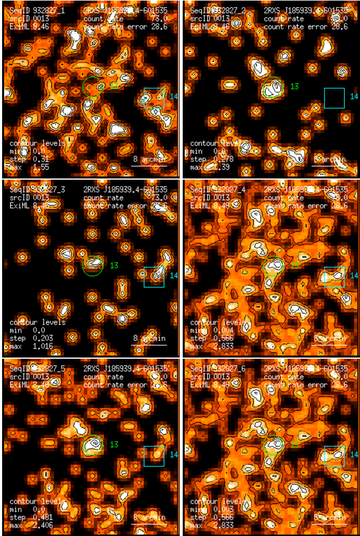
Figure 13: RASS 932827: detection 0013: band rate images, Gaussian filter: (1) PSPC channels 11 – 41, (2) 52 – 90, (3) 91 – 201, (4) 11 – 235, (5) 52 – 201, (6) 11 – 201. Broad band rates in counts/ks. Band rate contour levels in counts/ks/arcmin 2 .
