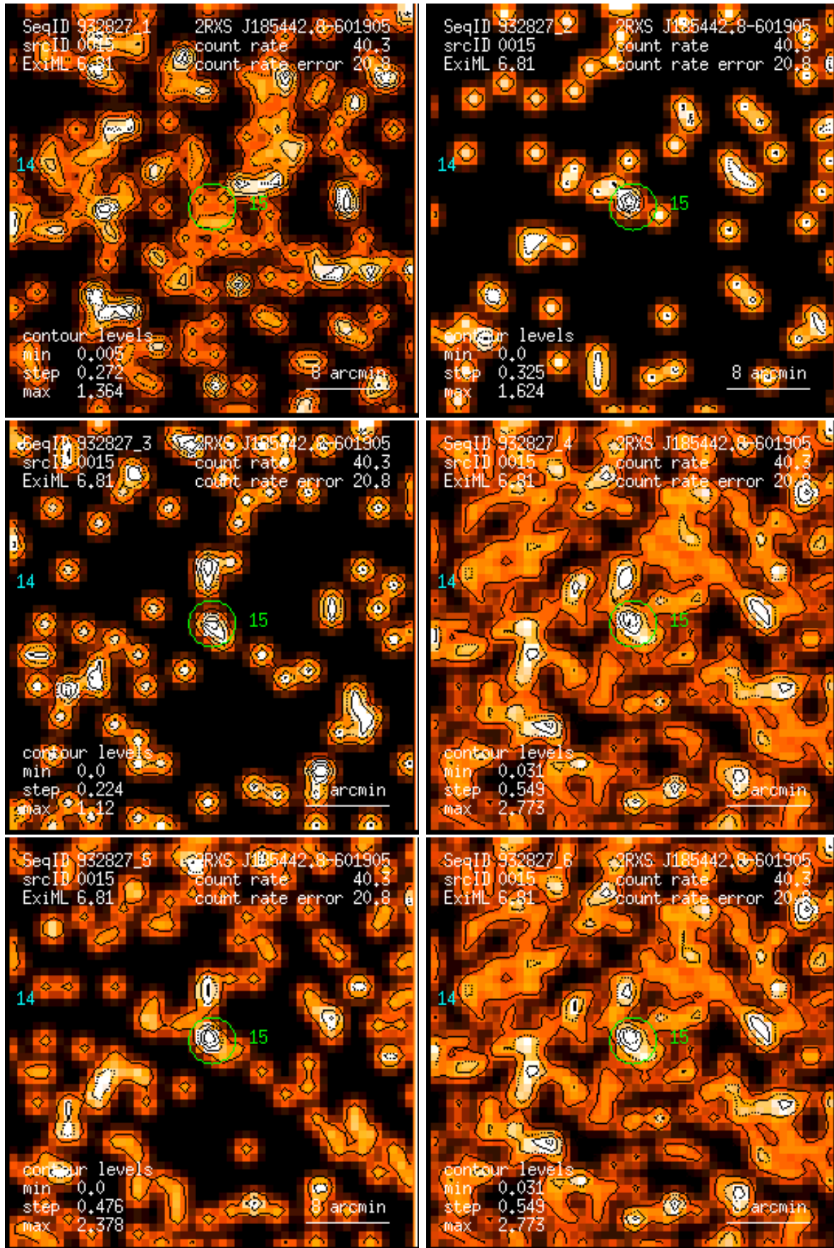
Figure 15: RASS 932827: detection 0015: band rate images, Gaussian filter: (1) PSPC channels 11 – 41, (2) 52 – 90, (3) 91 – 201, (4) 11 – 235, (5) 52 – 201, (6) 11 – 201. Broad band rates in counts/ks. Band rate contour levels in counts/ks/arcmin 2 .
