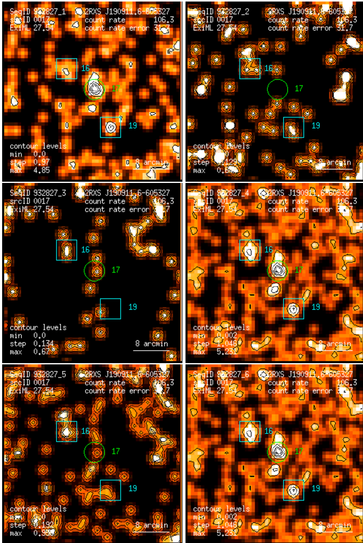
Figure 17: RASS 932827: detection 0017: band rate images, Gaussian filter: (1) PSPC channels 11 – 41, (2) 52 – 90, (3) 91 – 201, (4) 11 – 235, (5) 52 – 201, (6) 11 – 201. Broad band rates in counts/ks. Band rate contour levels in counts/ks/arcmin 2 .
