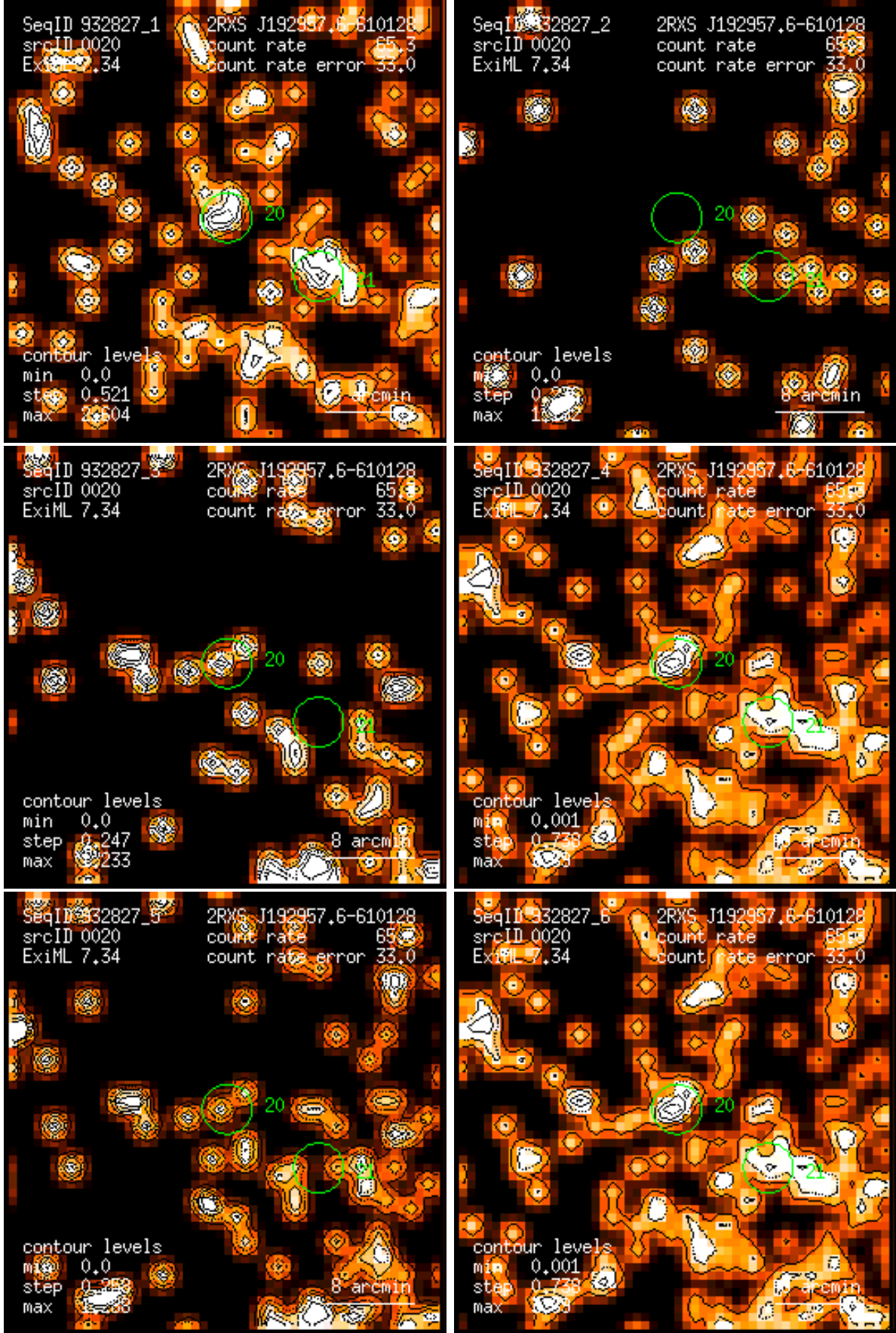
Figure 20: RASS 932827: detection 0020: band rate images, Gaussian filter: (1) PSPC channels 11 – 41, (2) 52 – 90, (3) 91 – 201, (4) 11 – 235, (5) 52 – 201, (6) 11 – 201. Broad band rates in counts/ks. Band rate contour levels in counts/ks/arcmin 2 .
