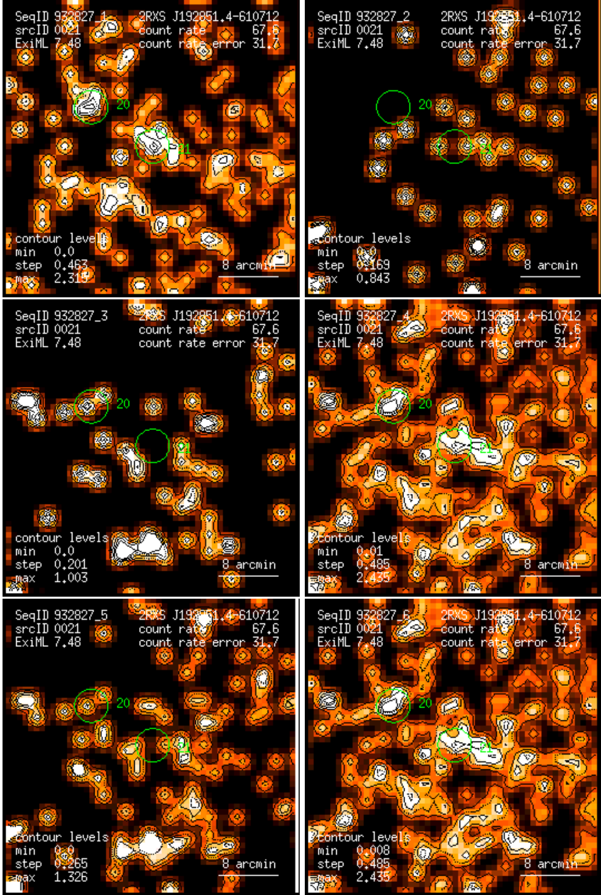
Figure 21: RASS 932827: detection 0021: band rate images, Gaussian filter: (1) PSPC channels 11 – 41, (2) 52 – 90, (3) 91 – 201, (4) 11 – 235, (5) 52 – 201, (6) 11 – 201. Broad band rates in counts/ks. Band rate contour levels in counts/ks/arcmin 2 .
