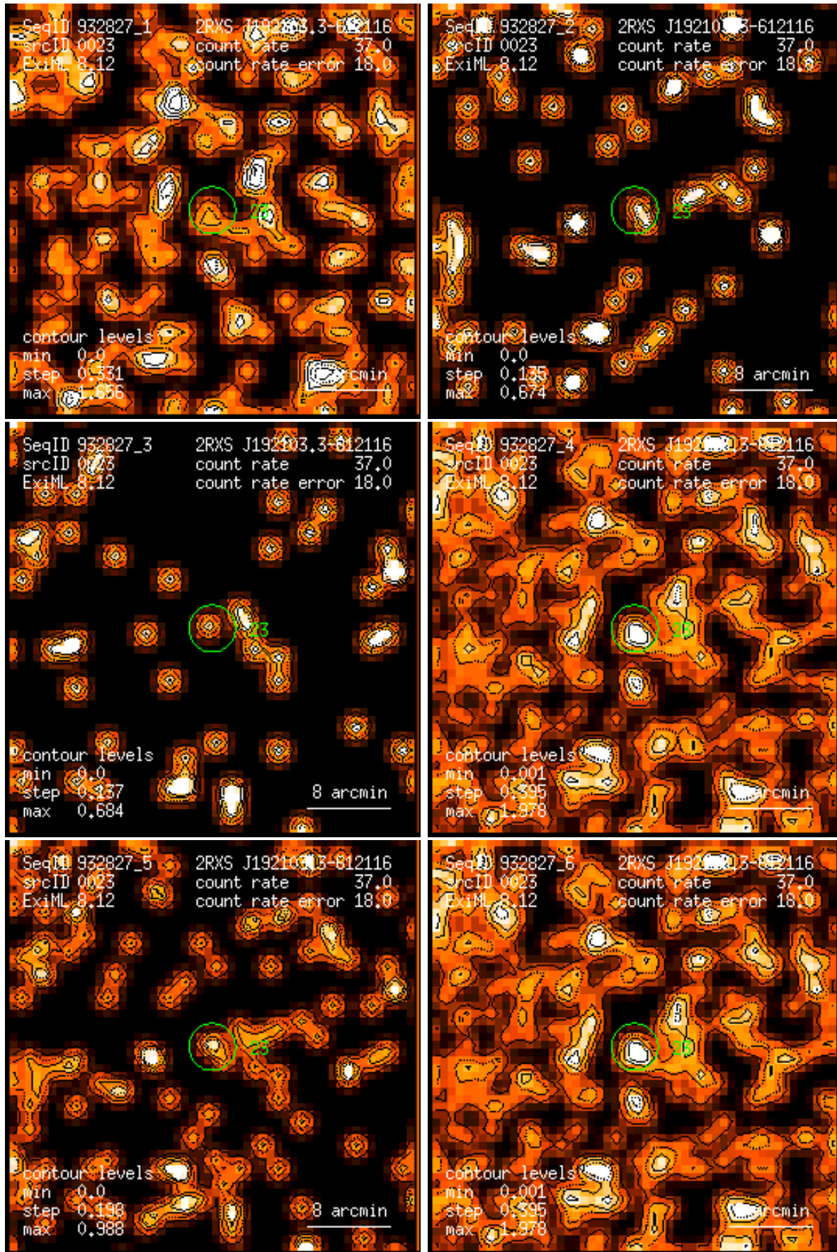
Figure 23: RASS 932827: detection 0023: band rate images, Gaussian filter: (1) PSPC channels 11 – 41, (2) 52 – 90, (3) 91 – 201, (4) 11 – 235, (5) 52 – 201, (6) 11 – 201. Broad band rates in counts/ks. Band rate contour levels in counts/ks/arcmin 2 .
