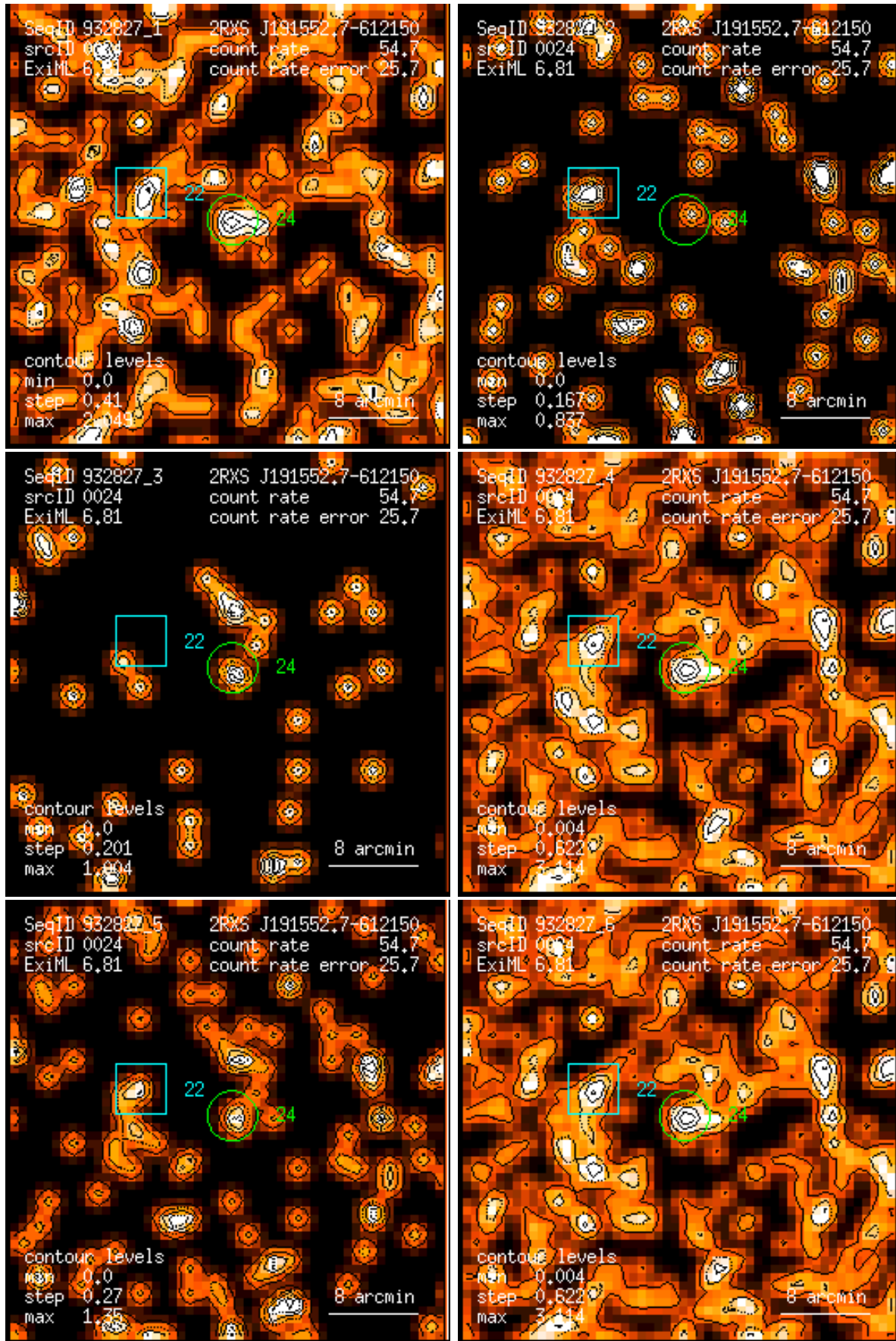
Figure 24: RASS 932827: detection 0024: band rate images, Gaussian filter: (1) PSPC channels 11 – 41, (2) 52 – 90, (3) 91 – 201, (4) 11 – 235, (5) 52 – 201, (6) 11 – 201. Broad band rates in counts/ks. Band rate contour levels in counts/ks/arcmin 2 .
