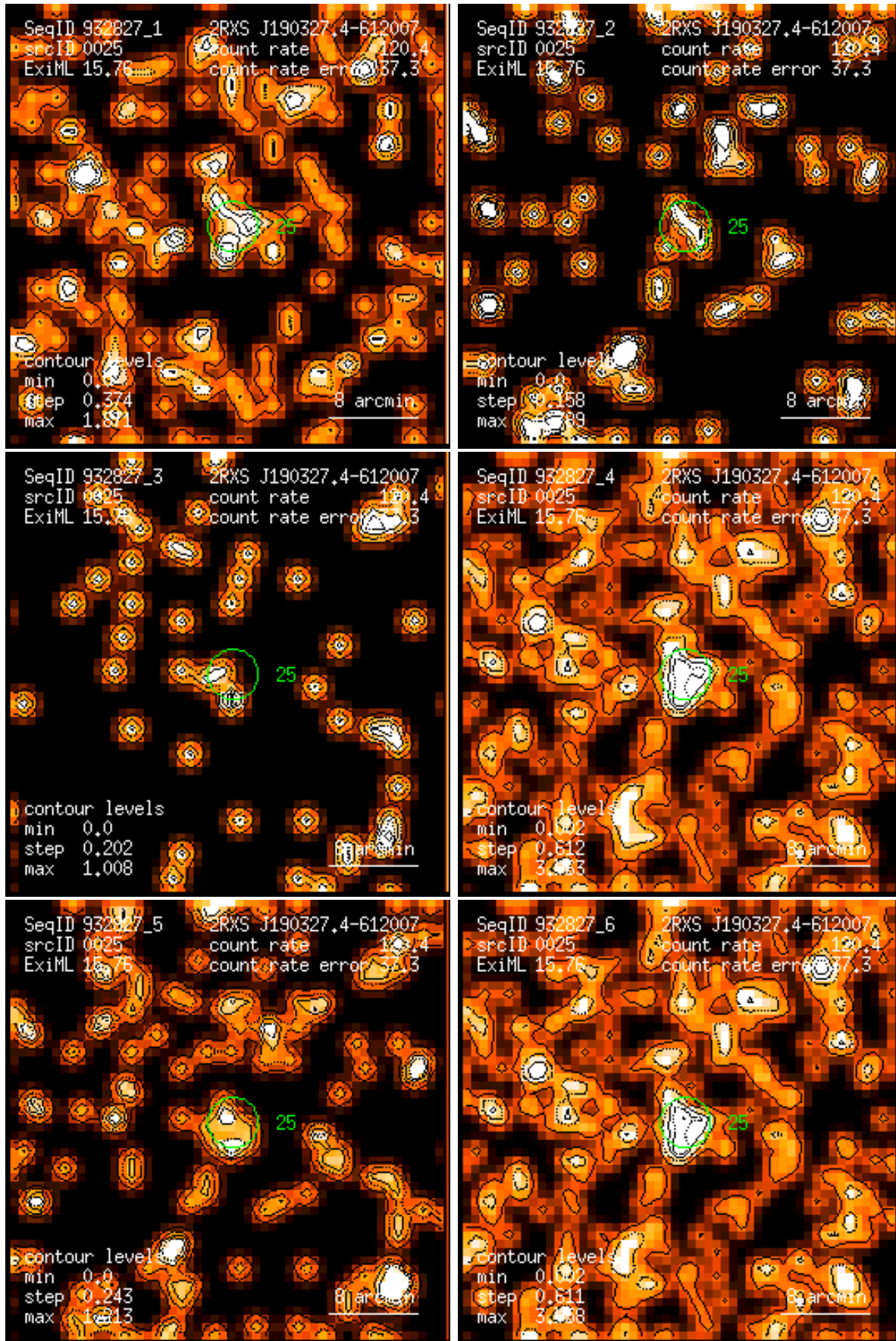
Figure 25: RASS 932827: detection 0025: band rate images, Gaussian filter: (1) PSPC channels 11 – 41, (2) 52 – 90, (3) 91 – 201, (4) 11 – 235, (5) 52 – 201, (6) 11 – 201. Broad band rates in counts/ks. Band rate contour levels in counts/ks/arcmin 2 .
