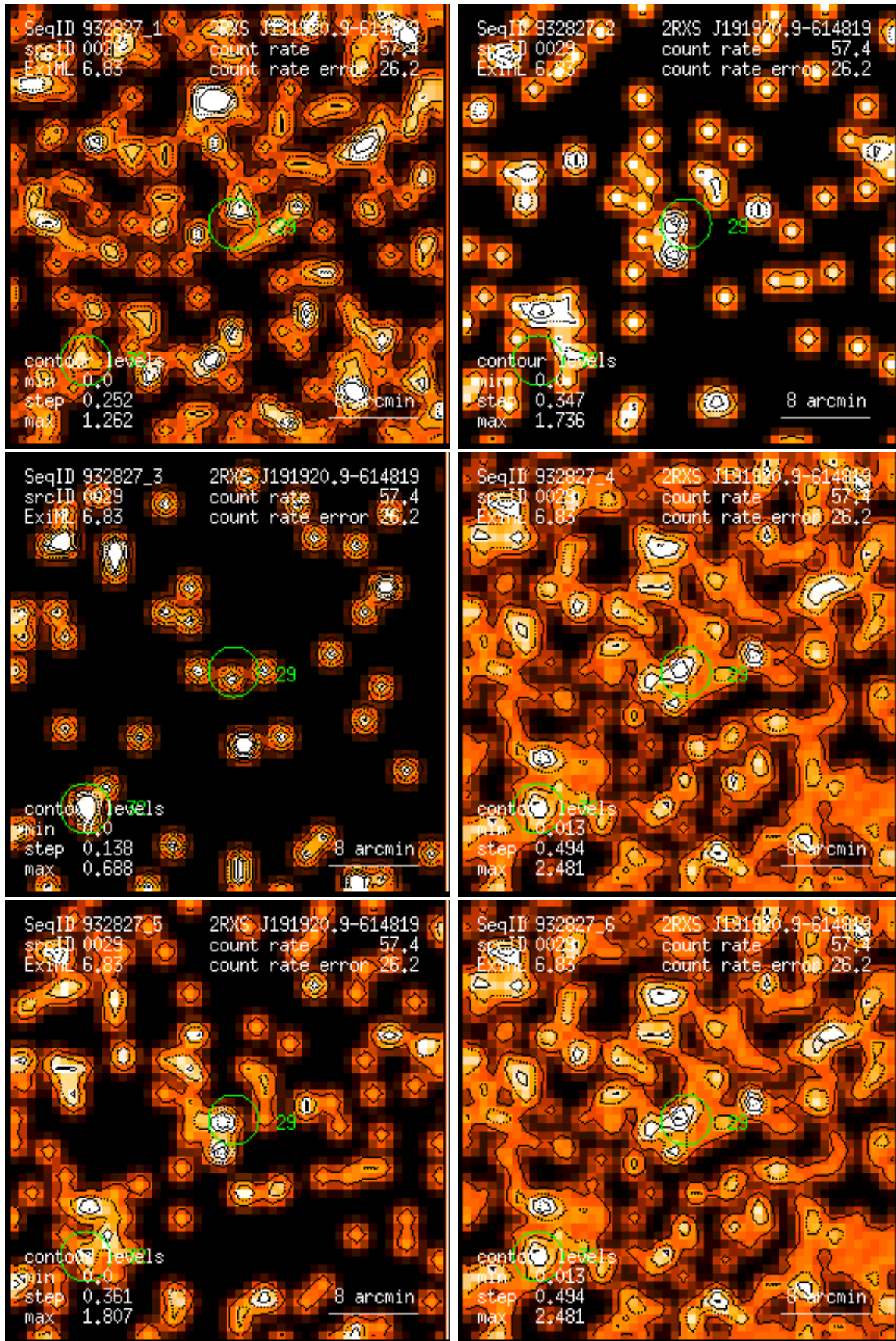
Figure 29: RASS 932827: detection 0029: band rate images, Gaussian filter: (1) PSPC channels 11 – 41, (2) 52 – 90, (3) 91 – 201, (4) 11 – 235, (5) 52 – 201, (6) 11 – 201. Broad band rates in counts/ks. Band rate contour levels in counts/ks/arcmin 2 .
