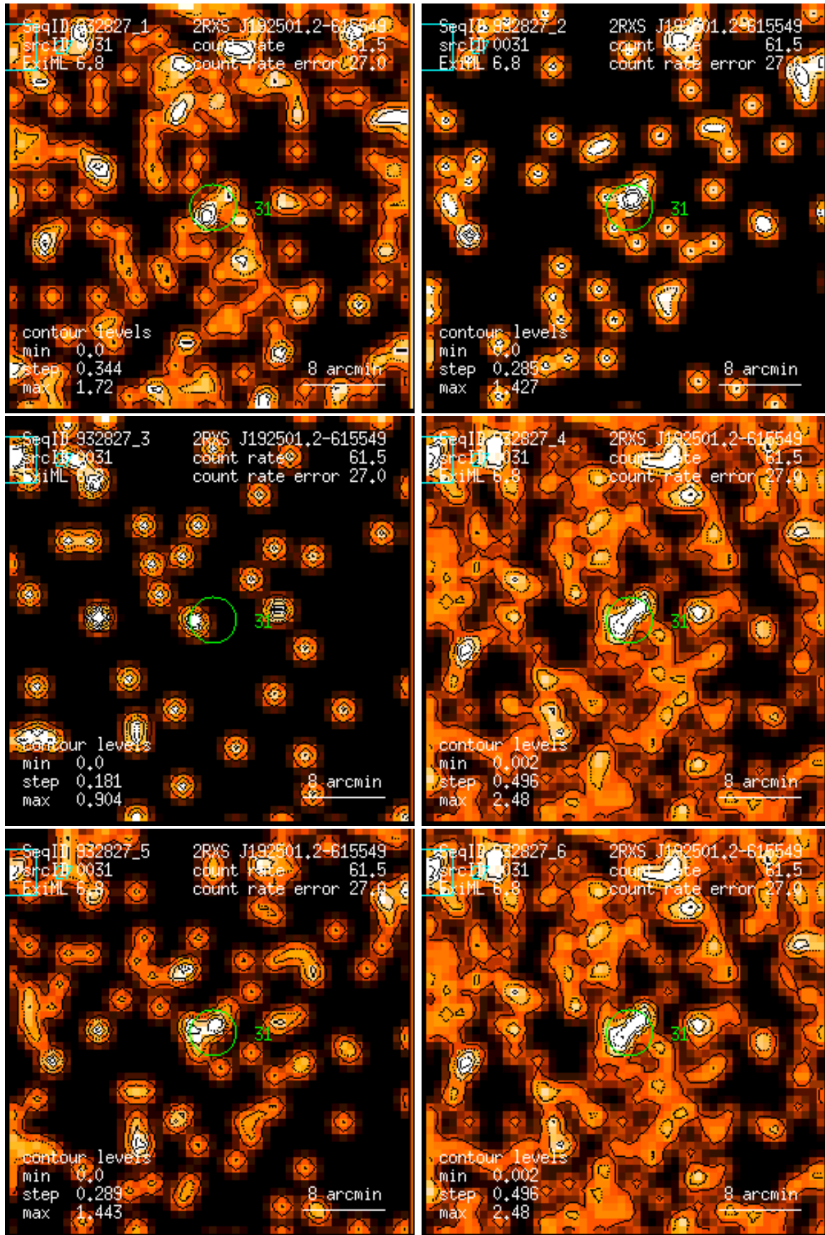
Figure 31: RASS 932827: detection 0031: band rate images, Gaussian filter: (1) PSPC channels 11 – 41, (2) 52 – 90, (3) 91 – 201, (4) 11 – 235, (5) 52 – 201, (6) 11 – 201. Broad band rates in counts/ks. Band rate contour levels in counts/ks/arcmin 2 .
