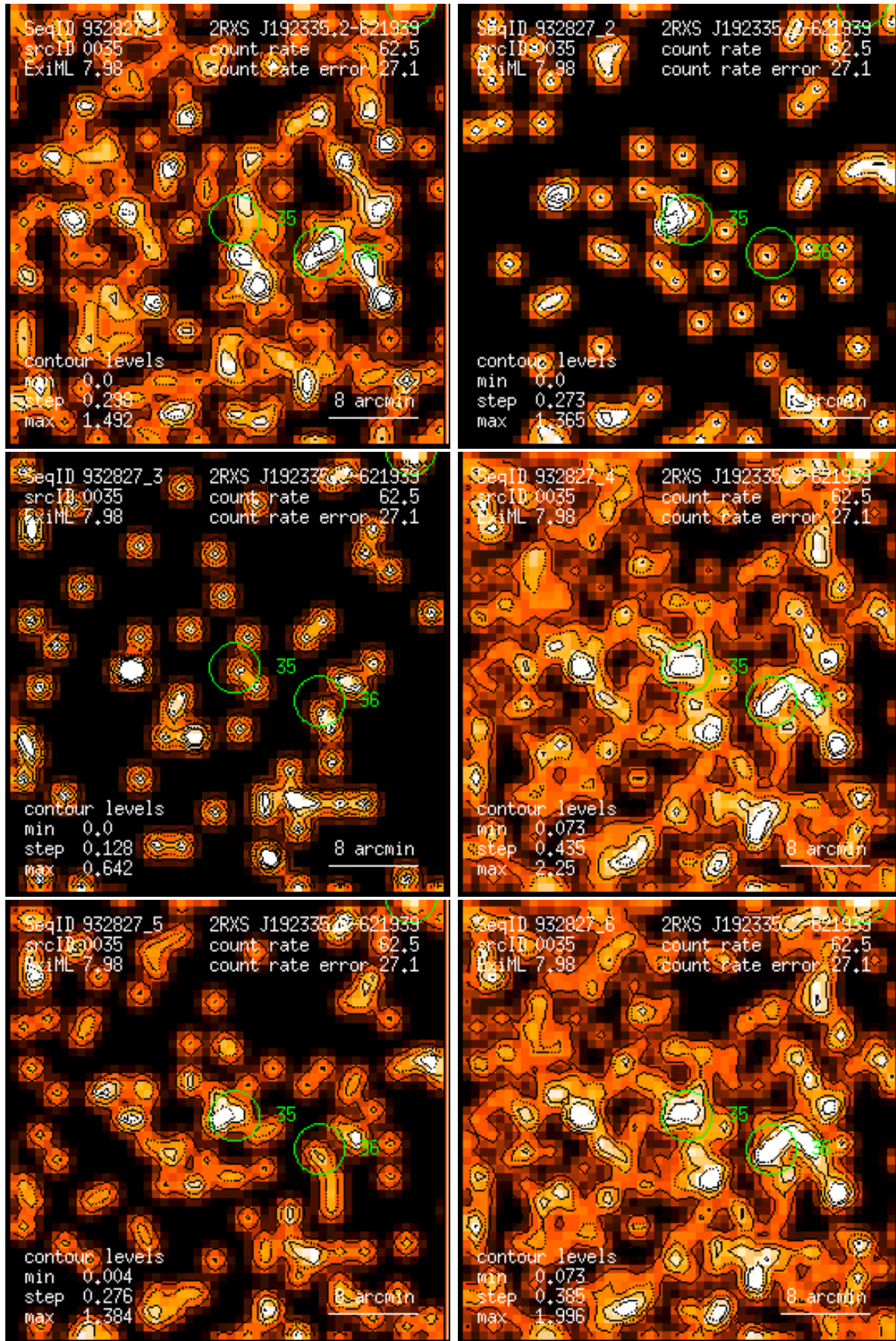
Figure 35: RASS 932827: detection 0035: band rate images, Gaussian filter: (1) PSPC channels 11 – 41, (2) 52 – 90, (3) 91 – 201, (4) 11 – 235, (5) 52 – 201, (6) 11 – 201. Broad band rates in counts/ks. Band rate contour levels in counts/ks/arcmin 2 .
