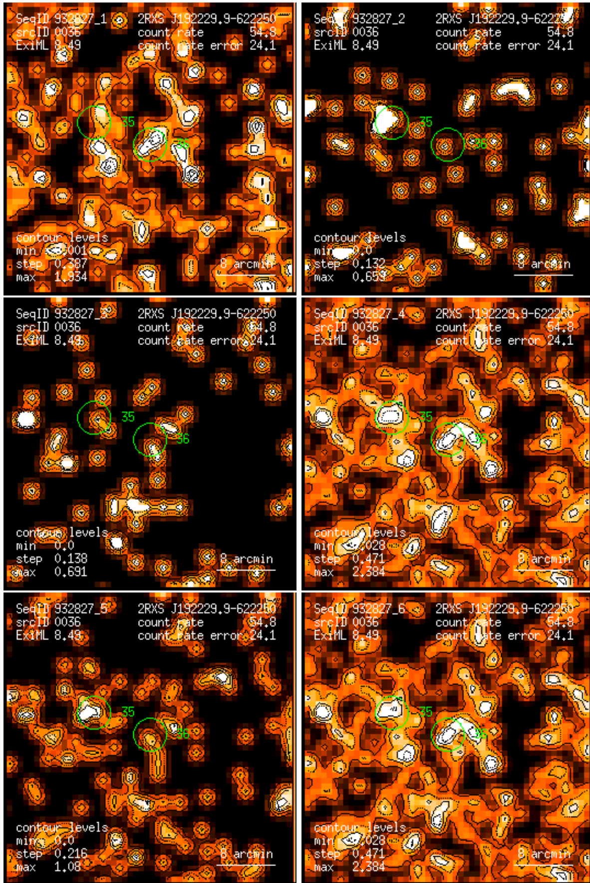
Figure 36: RASS 932827: detection 0036: band rate images, Gaussian filter: (1) PSPC channels 11 – 41, (2) 52 – 90, (3) 91 – 201, (4) 11 – 235, (5) 52 – 201, (6) 11 – 201. Broad band rates in counts/ks. Band rate contour levels in counts/ks/arcmin 2 .
