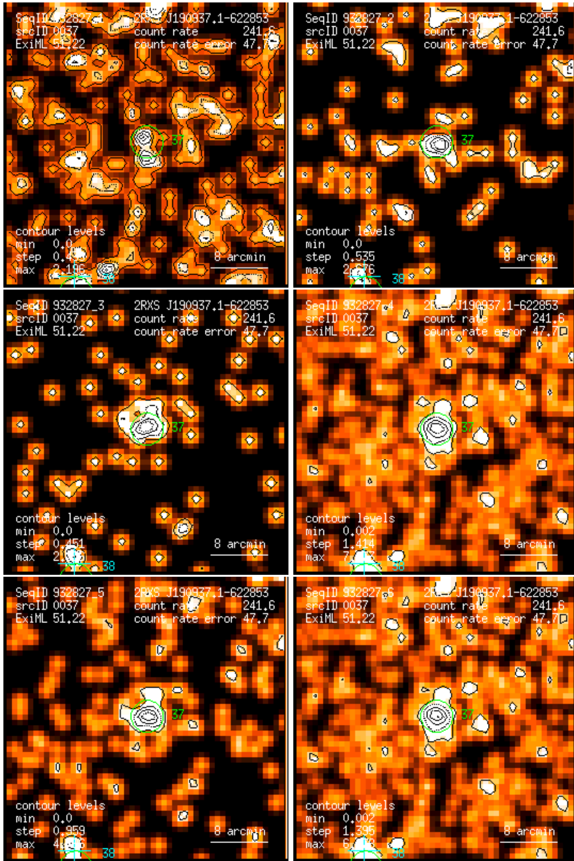
Figure 37: RASS 932827: detection 0037: band rate images, Gaussian filter: (1) PSPC channels 11 – 41, (2) 52 – 90, (3) 91 – 201, (4) 11 – 235, (5) 52 – 201, (6) 11 – 201. Broad band rates in counts/ks. Band rate contour levels in counts/ks/arcmin 2 .
