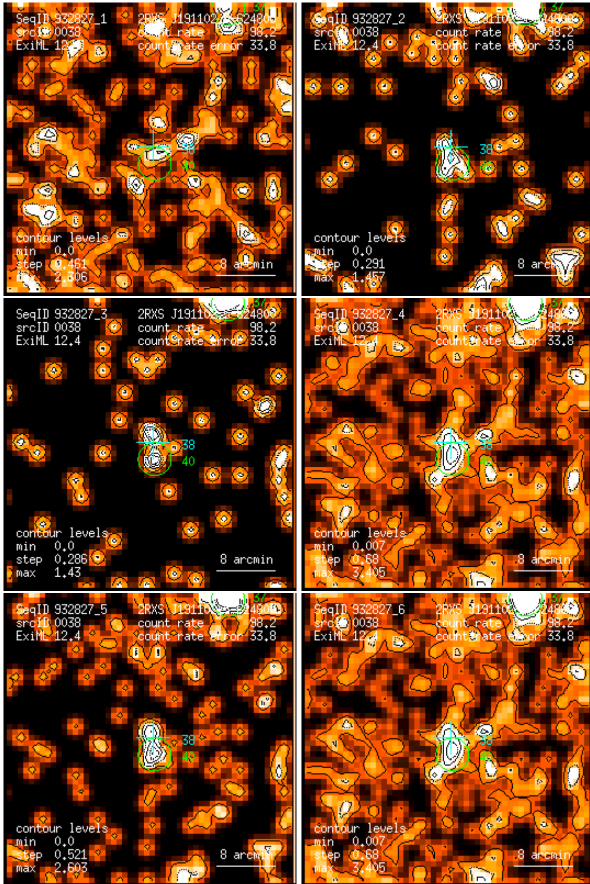
Figure 38: RASS 932827: detection 0038: band rate images, Gaussian filter: (1) PSPC channels 11 – 41, (2) 52 – 90, (3) 91 – 201, (4) 11 – 235, (5) 52 – 201, (6) 11 – 201. Broad band rates in counts/ks. Band rate contour levels in counts/ks/arcmin 2 .
