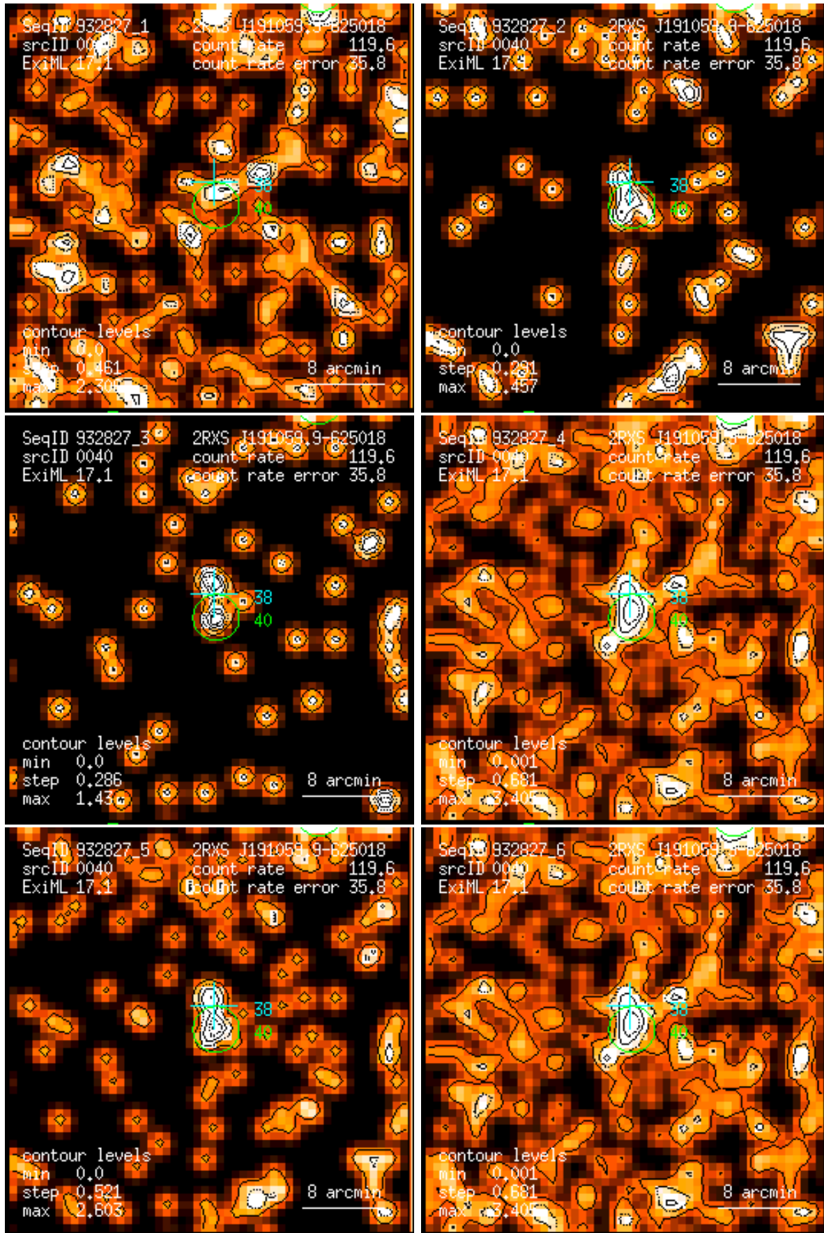
Figure 40: RASS 932827: detection 0040: band rate images, Gaussian filter: (1) PSPC channels 11 – 41, (2) 52 – 90, (3) 91 – 201, (4) 11 – 235, (5) 52 – 201, (6) 11 – 201. Broad band rates in counts/ks. Band rate contour levels in counts/ks/arcmin 2 .
