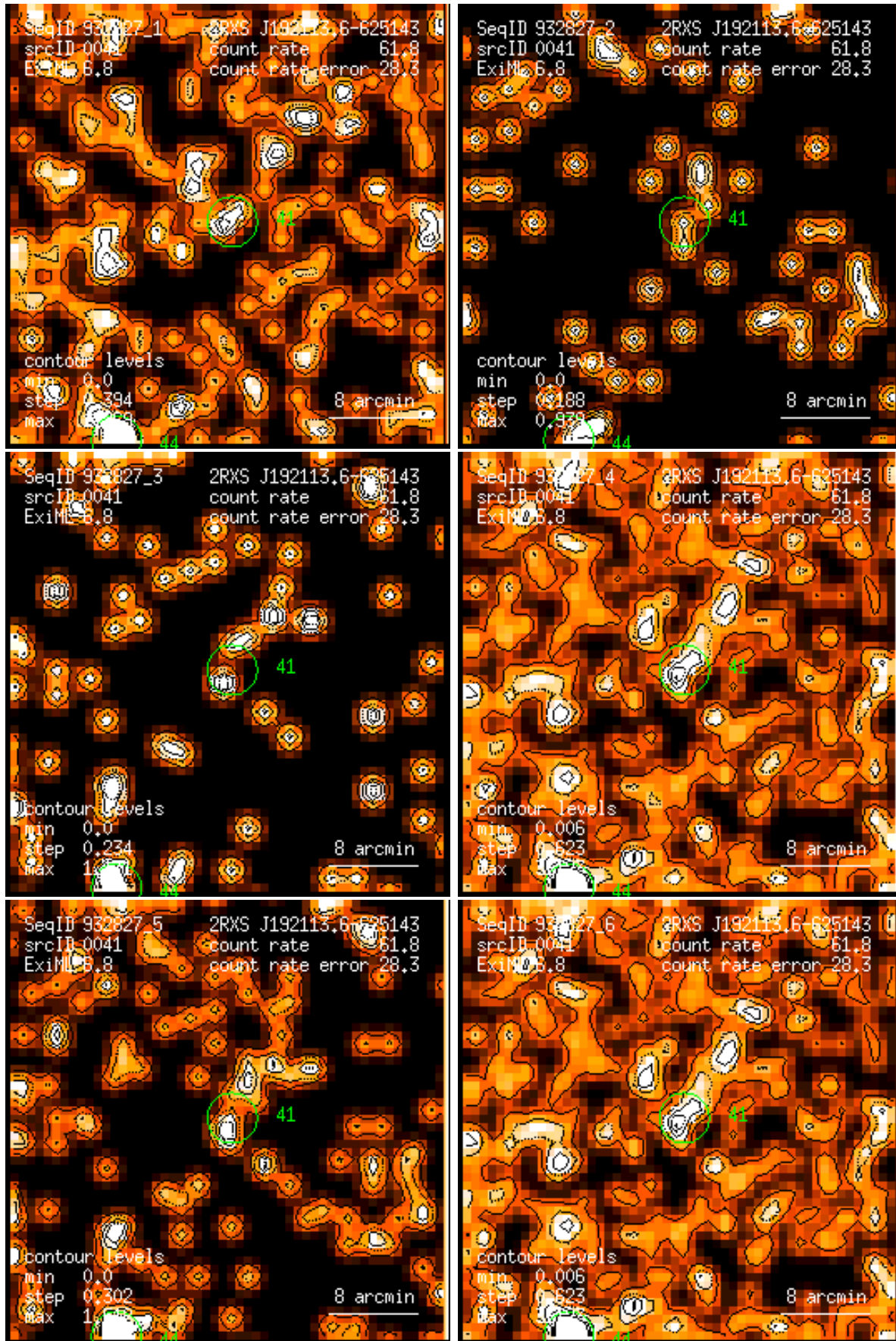
Figure 41: RASS 932827: detection 0041: band rate images, Gaussian filter: (1) PSPC channels 11 – 41, (2) 52 – 90, (3) 91 – 201, (4) 11 – 235, (5) 52 – 201, (6) 11 – 201. Broad band rates in counts/ks. Band rate contour levels in counts/ks/arcmin 2 .
