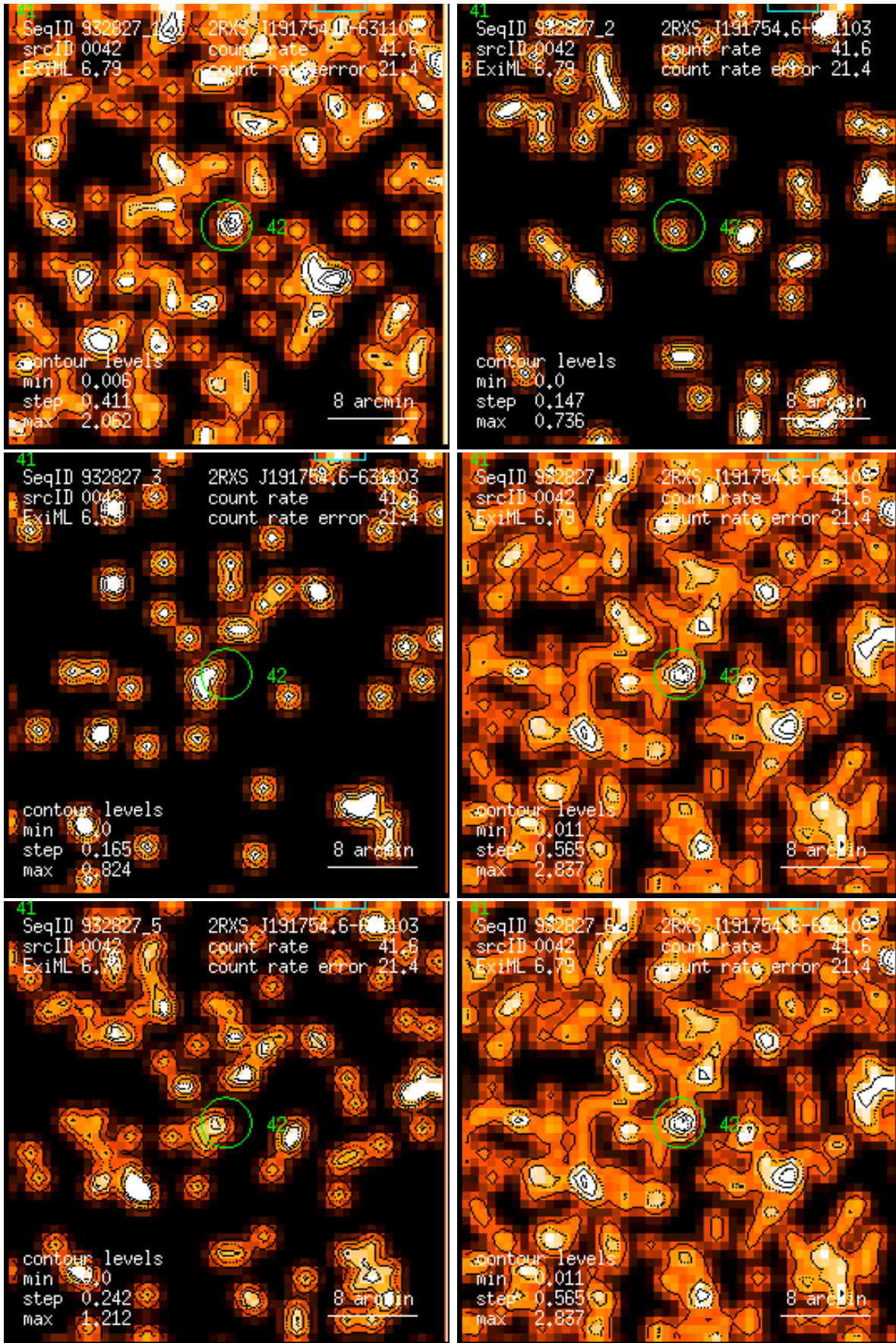
Figure 42: RASS 932827: detection 0042: band rate images, Gaussian filter: (1) PSPC channels 11 – 41, (2) 52 – 90, (3) 91 – 201, (4) 11 – 235, (5) 52 – 201, (6) 11 – 201. Broad band rates in counts/ks. Band rate contour levels in counts/ks/arcmin 2 .
