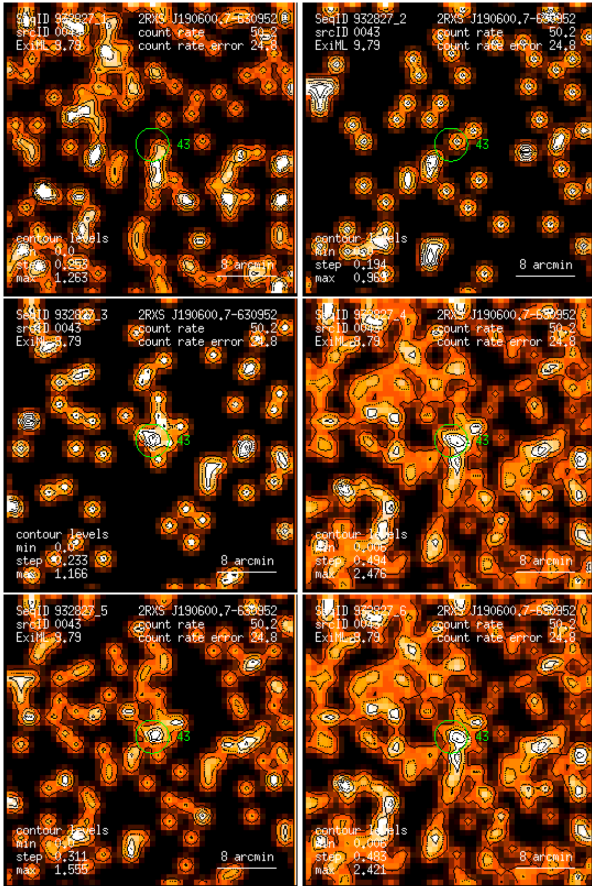
Figure 43: RASS 932827: detection 0043: band rate images, Gaussian filter: (1) PSPC channels 11 – 41, (2) 52 – 90, (3) 91 – 201, (4) 11 – 235, (5) 52 – 201, (6) 11 – 201. Broad band rates in counts/ks. Band rate contour levels in counts/ks/arcmin 2 .
