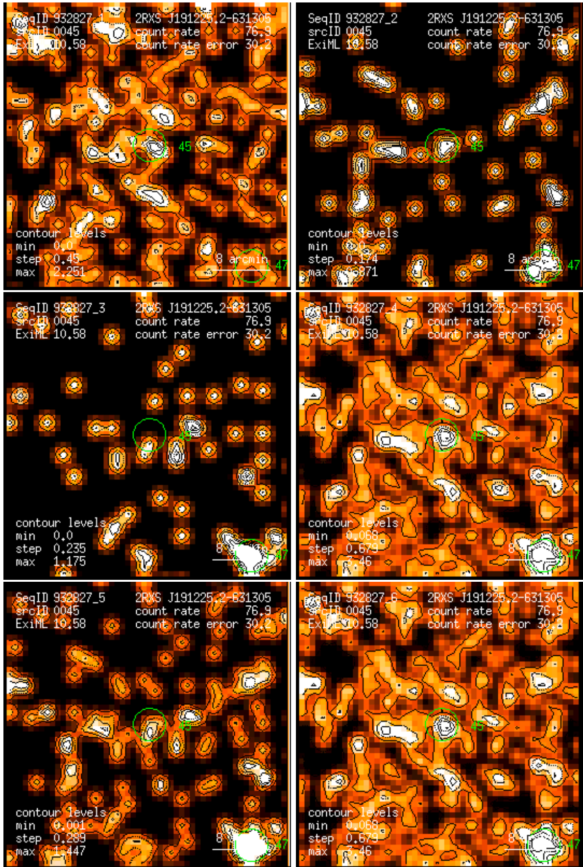
Figure 45: RASS 932827: detection 0045: band rate images, Gaussian filter: (1) PSPC channels 11 – 41, (2) 52 – 90, (3) 91 – 201, (4) 11 – 235, (5) 52 – 201, (6) 11 – 201. Broad band rates in counts/ks. Band rate contour levels in counts/ks/arcmin 2 .
