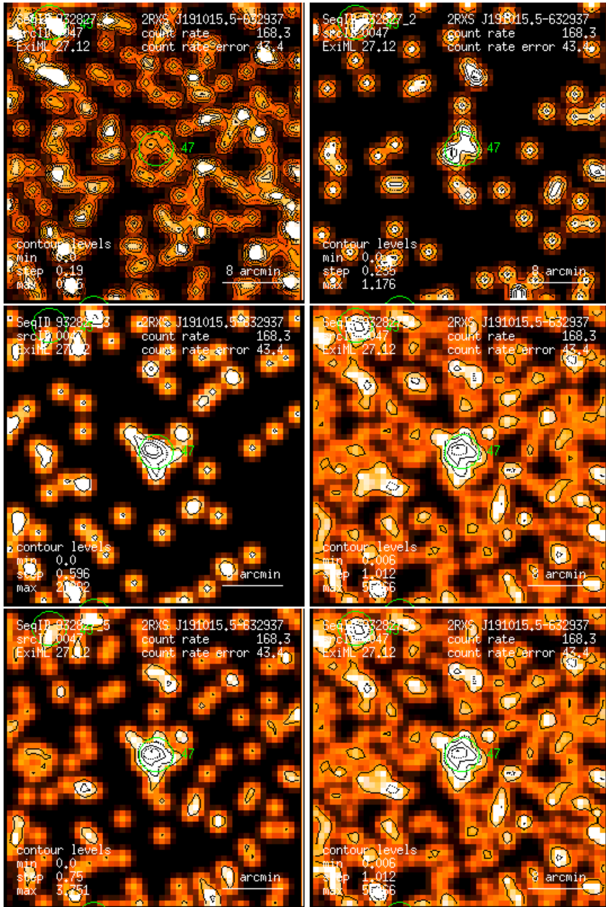
Figure 47: RASS 932827: detection 0047: band rate images, Gaussian filter: (1) PSPC channels 11 – 41, (2) 52 – 90, (3) 91 – 201, (4) 11 – 235, (5) 52 – 201, (6) 11 – 201. Broad band rates in counts/ks. Band rate contour levels in counts/ks/arcmin 2 .
