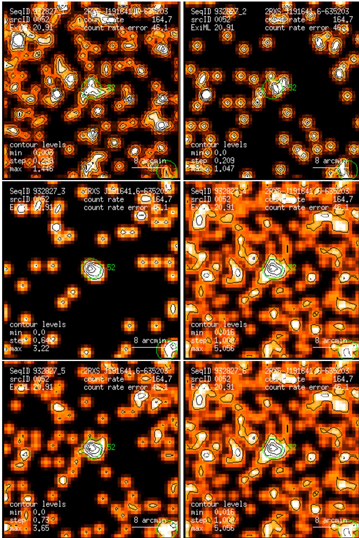
Figure 52: RASS 932827: detection 0052: band rate images, Gaussian filter: (1) PSPC channels 11 – 41, (2) 52 – 90, (3) 91 – 201, (4) 11 – 235, (5) 52 – 201, (6) 11 – 201. Broad band rates in counts/ks. Band rate contour levels in counts/ks/arcmin 2 .
