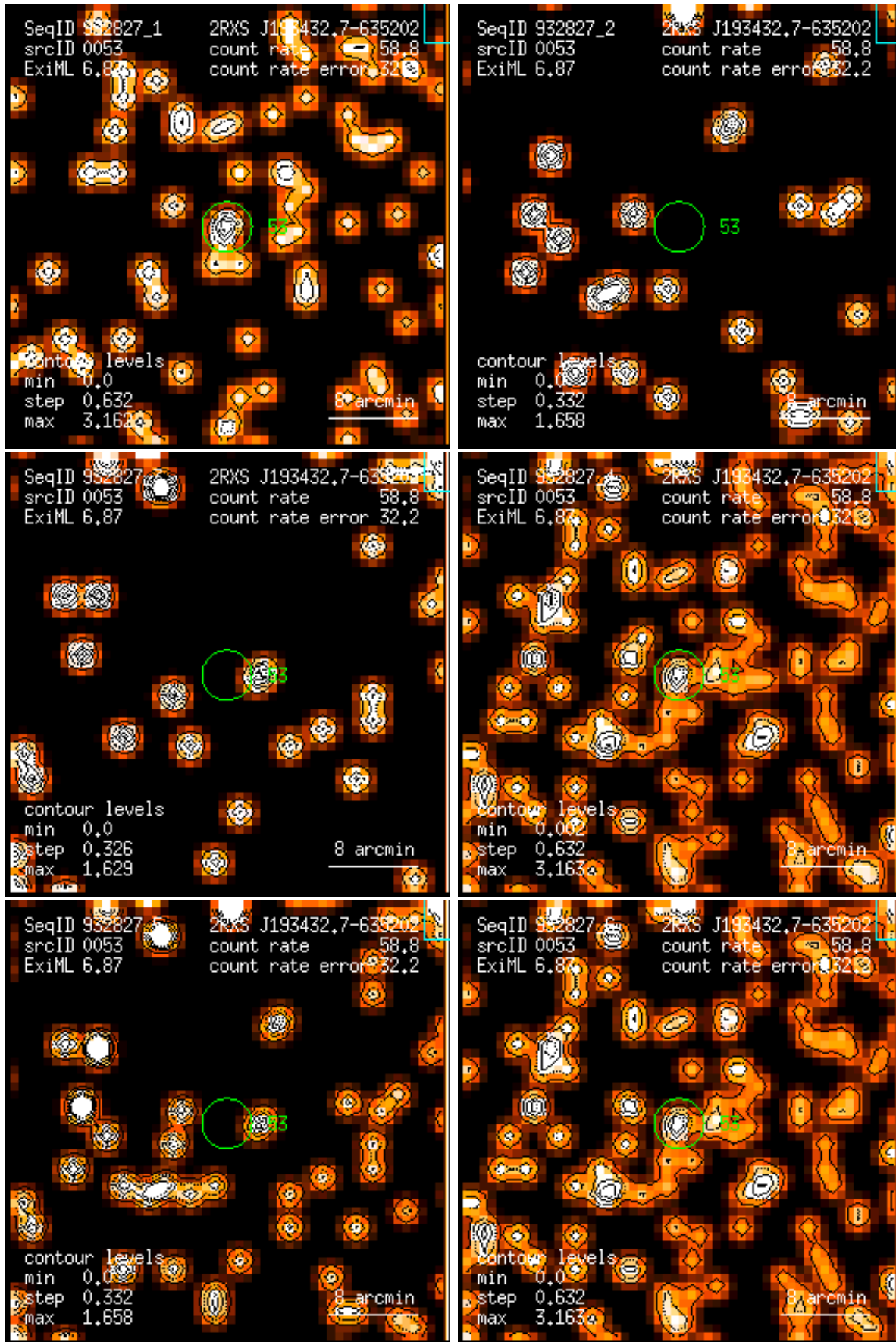
Figure 53: RASS 932827: detection 0053: band rate images, Gaussian filter: (1) PSPC channels 11 – 41, (2) 52 – 90, (3) 91 – 201, (4) 11 – 235, (5) 52 – 201, (6) 11 – 201. Broad band rates in counts/ks. Band rate contour levels in counts/ks/arcmin 2 .
