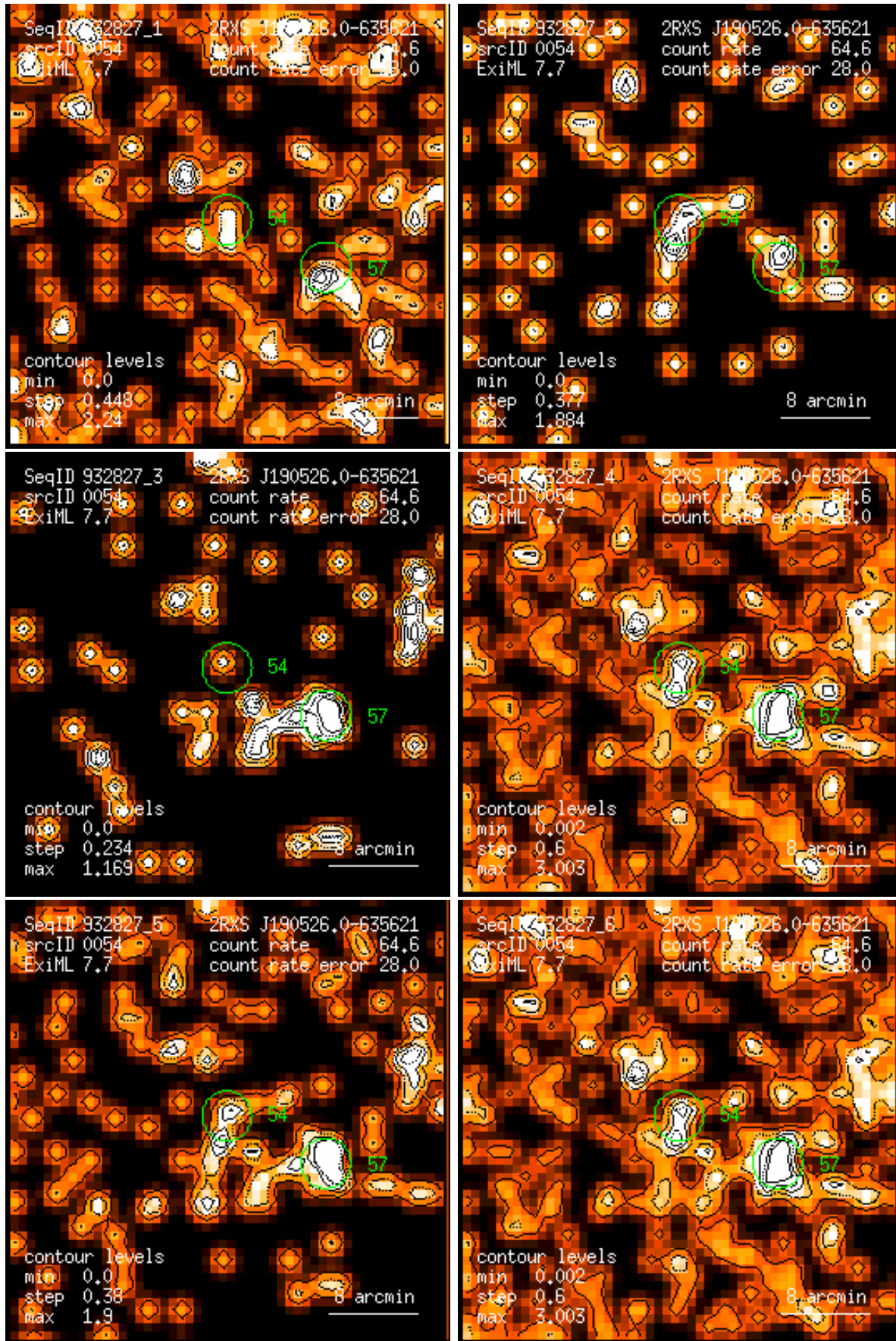
Figure 54: RASS 932827: detection 0054: band rate images, Gaussian filter: (1) PSPC channels 11 – 41, (2) 52 – 90, (3) 91 – 201, (4) 11 – 235, (5) 52 – 201, (6) 11 – 201. Broad band rates in counts/ks. Band rate contour levels in counts/ks/arcmin 2 .
