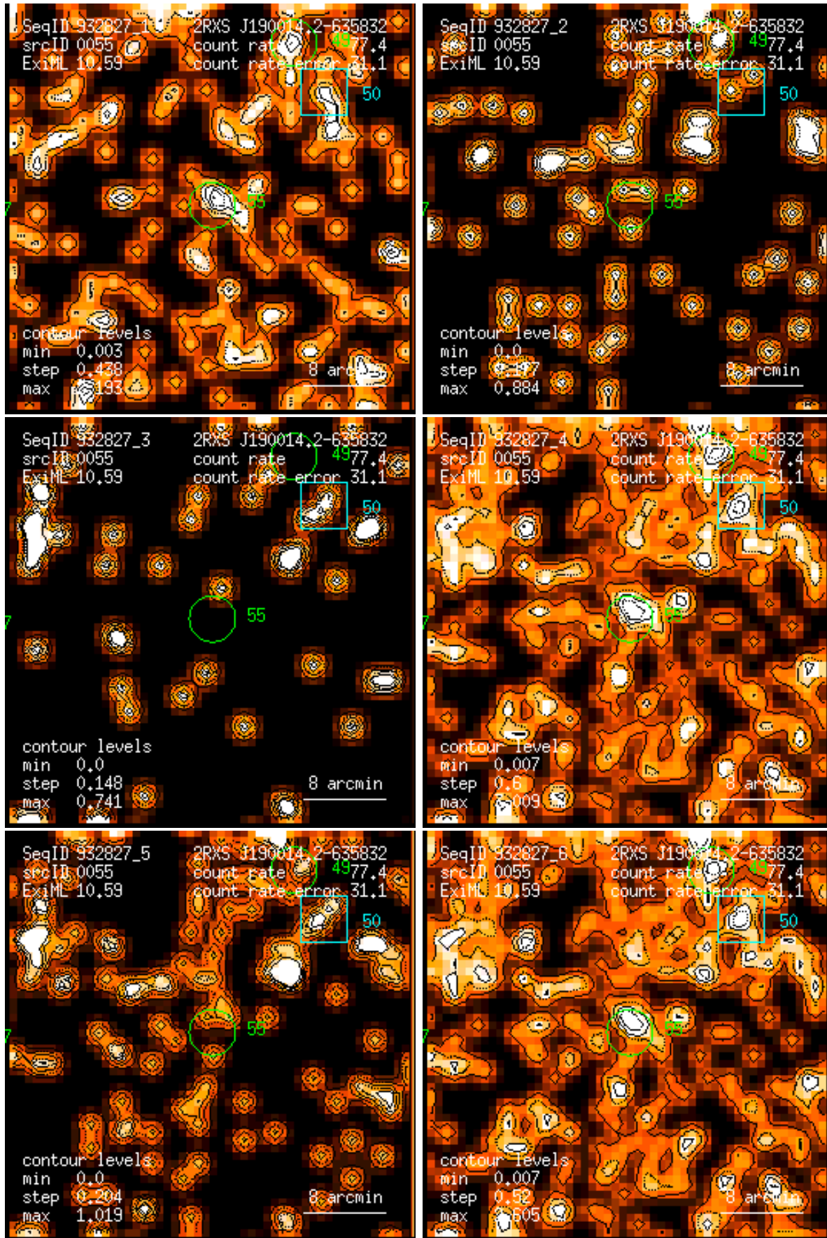
Figure 55: RASS 932827: detection 0055: band rate images, Gaussian filter: (1) PSPC channels 11 – 41, (2) 52 – 90, (3) 91 – 201, (4) 11 – 235, (5) 52 – 201, (6) 11 – 201. Broad band rates in counts/ks. Band rate contour levels in counts/ks/arcmin 2 .
