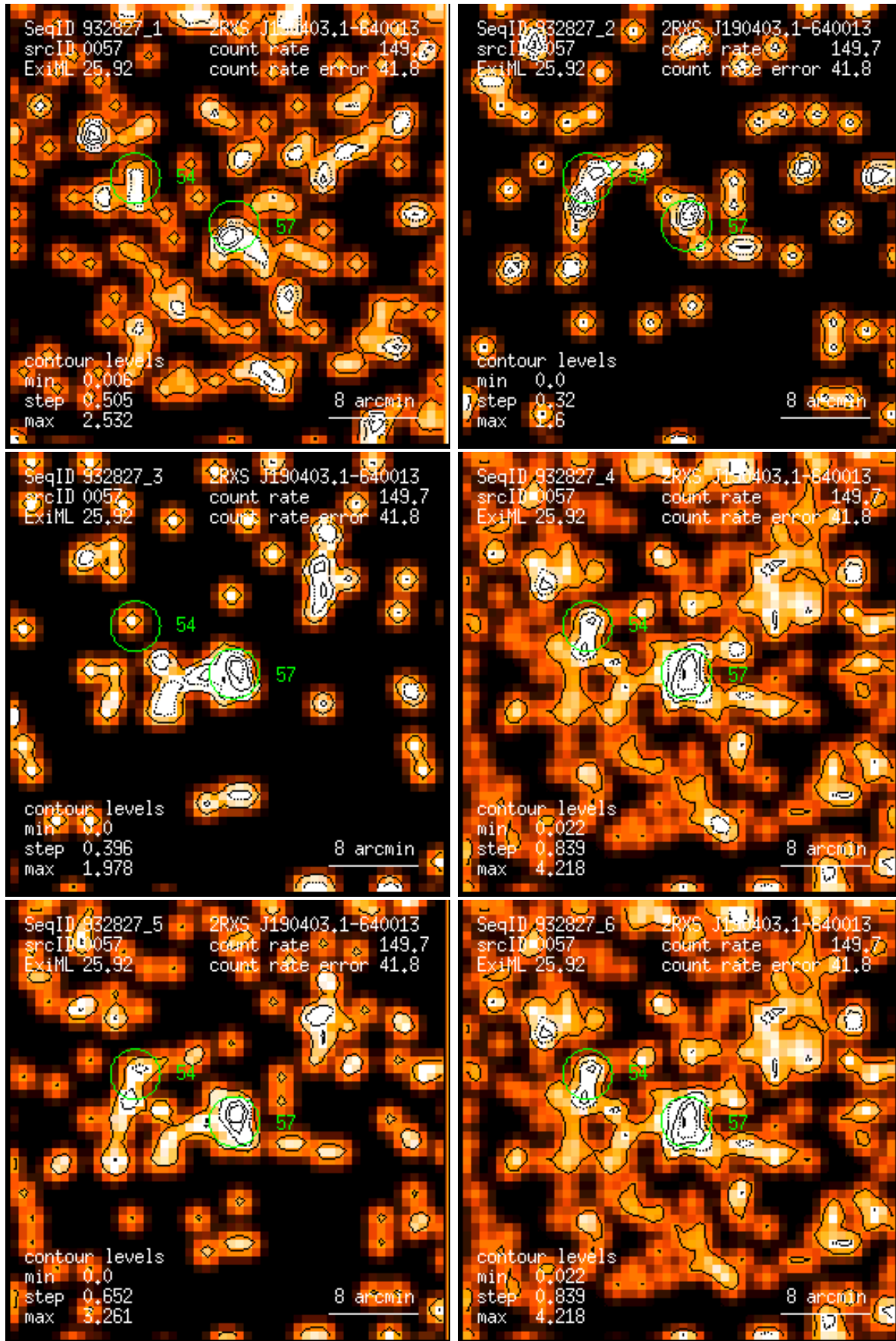
Figure 57: RASS 932827: detection 0057: band rate images, Gaussian filter: (1) PSPC channels 11 – 41, (2) 52 – 90, (3) 91 – 201, (4) 11 – 235, (5) 52 – 201, (6) 11 – 201. Broad band rates in counts/ks. Band rate contour levels in counts/ks/arcmin 2 .
