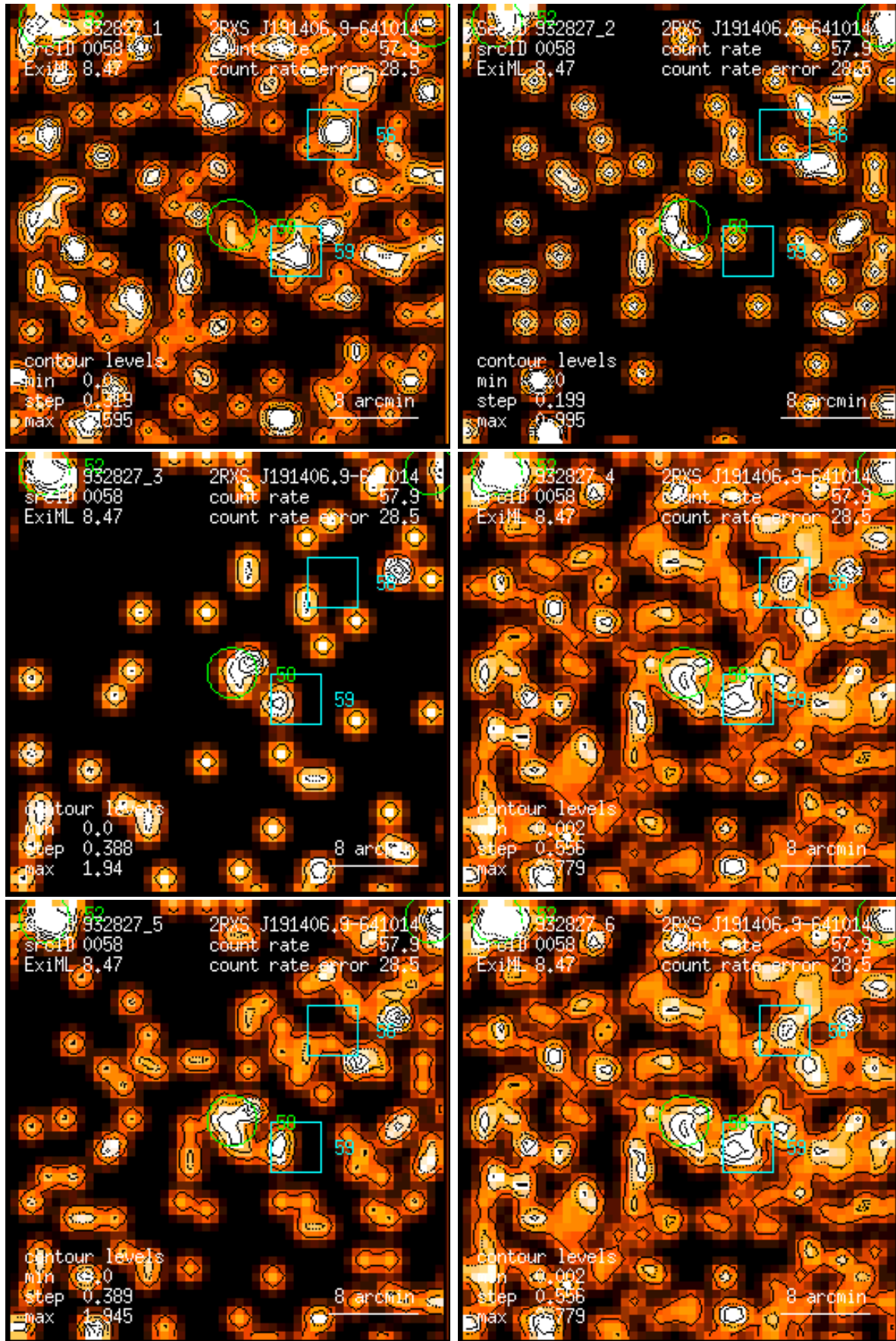
Figure 58: RASS 932827: detection 0058: band rate images, Gaussian filter: (1) PSPC channels 11 – 41, (2) 52 – 90, (3) 91 – 201, (4) 11 – 235, (5) 52 – 201, (6) 11 – 201. Broad band rates in counts/ks. Band rate contour levels in counts/ks/arcmin 2 .
