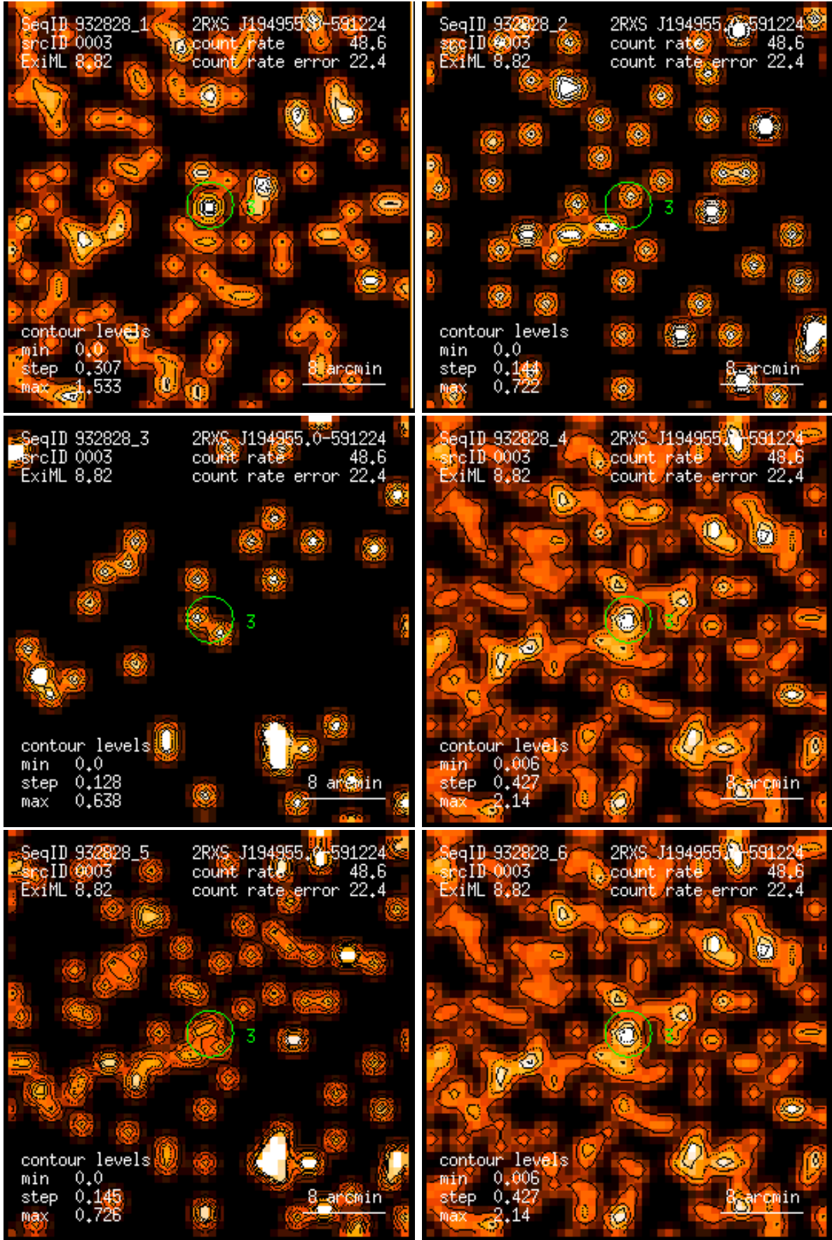
Figure 3: RASS 932828: detection 0003: band rate images, Gaussian filter: (1) PSPC channels 11 – 41, (2) 52 – 90, (3) 91 – 201, (4) 11 – 235, (5) 52 – 201, (6) 11 – 201. Broad band rates in counts/ks. Band rate contour levels in counts/ks/arcmin 2 .
