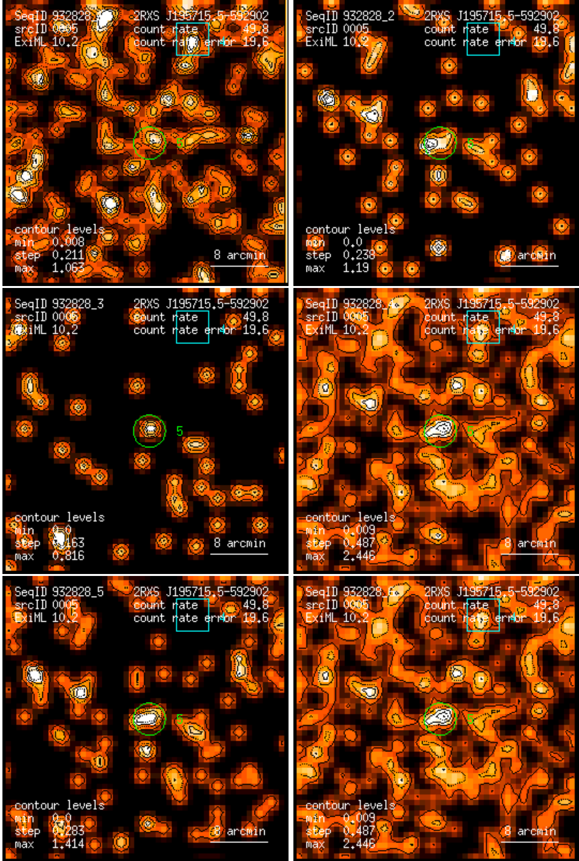
Figure 5: RASS 932828: detection 0005: band rate images, Gaussian filter: (1) PSPC channels 11 – 41, (2) 52 – 90, (3) 91 – 201, (4) 11 – 235, (5) 52 – 201, (6) 11 – 201. Broad band rates in counts/ks. Band rate contour levels in counts/ks/arcmin 2 .
