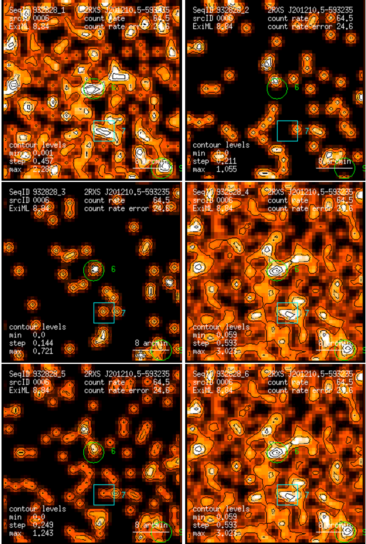
Figure 6: RASS 932828: detection 0006: band rate images, Gaussian filter: (1) PSPC channels 11 – 41, (2) 52 – 90, (3) 91 – 201, (4) 11 – 235, (5) 52 – 201, (6) 11 – 201. Broad band rates in counts/ks. Band rate contour levels in counts/ks/arcmin 2 .
