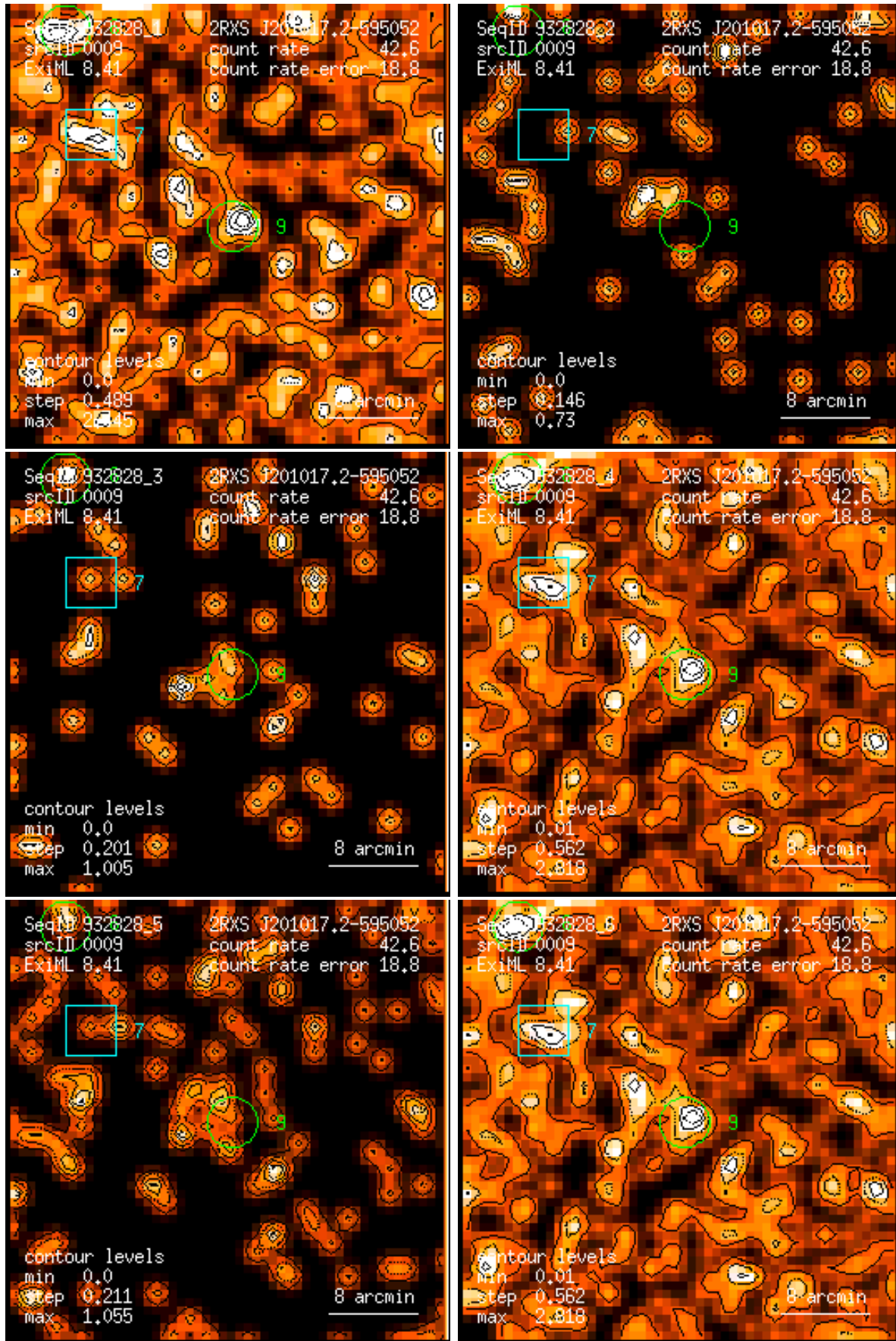
Figure 9: RASS 932828: detection 0009: band rate images, Gaussian filter: (1) PSPC channels 11 – 41, (2) 52 – 90, (3) 91 – 201, (4) 11 – 235, (5) 52 – 201, (6) 11 – 201. Broad band rates in counts/ks. Band rate contour levels in counts/ks/arcmin 2 .
