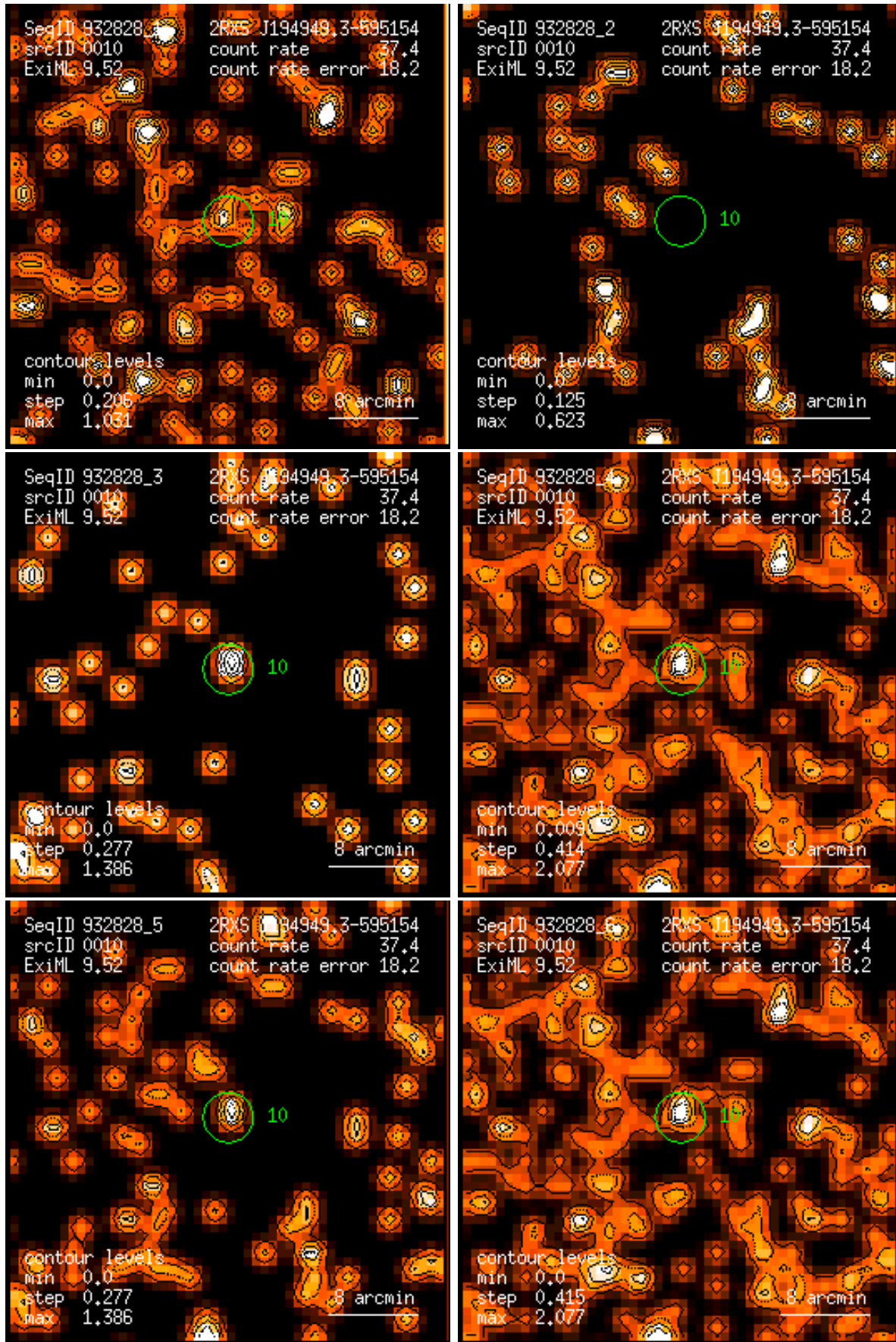
Figure 10: RASS 932828: detection 0010: band rate images, Gaussian filter: (1) PSPC channels 11 – 41, (2) 52 – 90, (3) 91 – 201, (4) 11 – 235, (5) 52 – 201, (6) 11 – 201. Broad band rates in counts/ks. Band rate contour levels in counts/ks/arcmin 2 .
