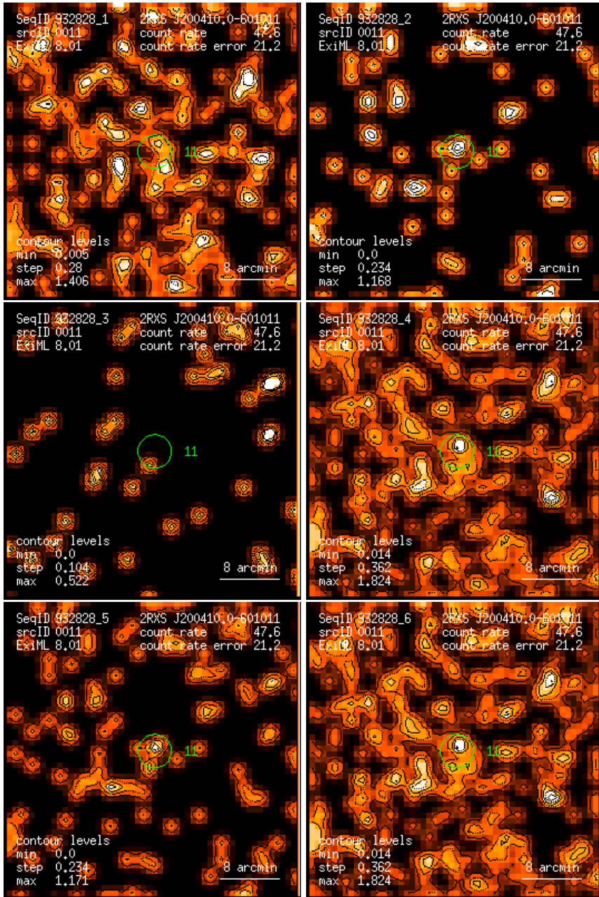
Figure 11: RASS 932828: detection 0011: band rate images, Gaussian filter: (1) PSPC channels 11 – 41, (2) 52 – 90, (3) 91 – 201, (4) 11 – 235, (5) 52 – 201, (6) 11 – 201. Broad band rates in counts/ks. Band rate contour levels in counts/ks/arcmin 2 .
