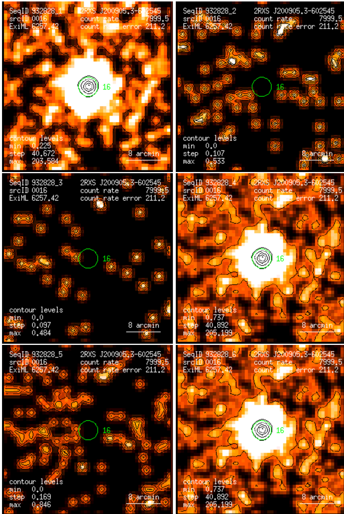
Figure 16: RASS 932828: detection 0016: band rate images, Gaussian filter: (1) PSPC channels 11 – 41, (2) 52 – 90, (3) 91 – 201, (4) 11 – 235, (5) 52 – 201, (6) 11 – 201. Broad band rates in counts/ks. Band rate contour levels in counts/ks/arcmin 2 .
