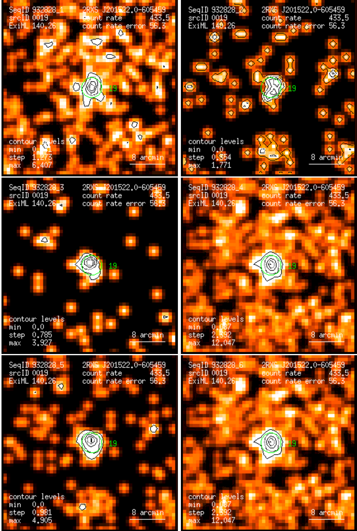
Figure 19: RASS 932828: detection 0019: band rate images, Gaussian filter: (1) PSPC channels 11 – 41, (2) 52 – 90, (3) 91 – 201, (4) 11 – 235, (5) 52 – 201, (6) 11 – 201. Broad band rates in counts/ks. Band rate contour levels in counts/ks/arcmin 2 .
