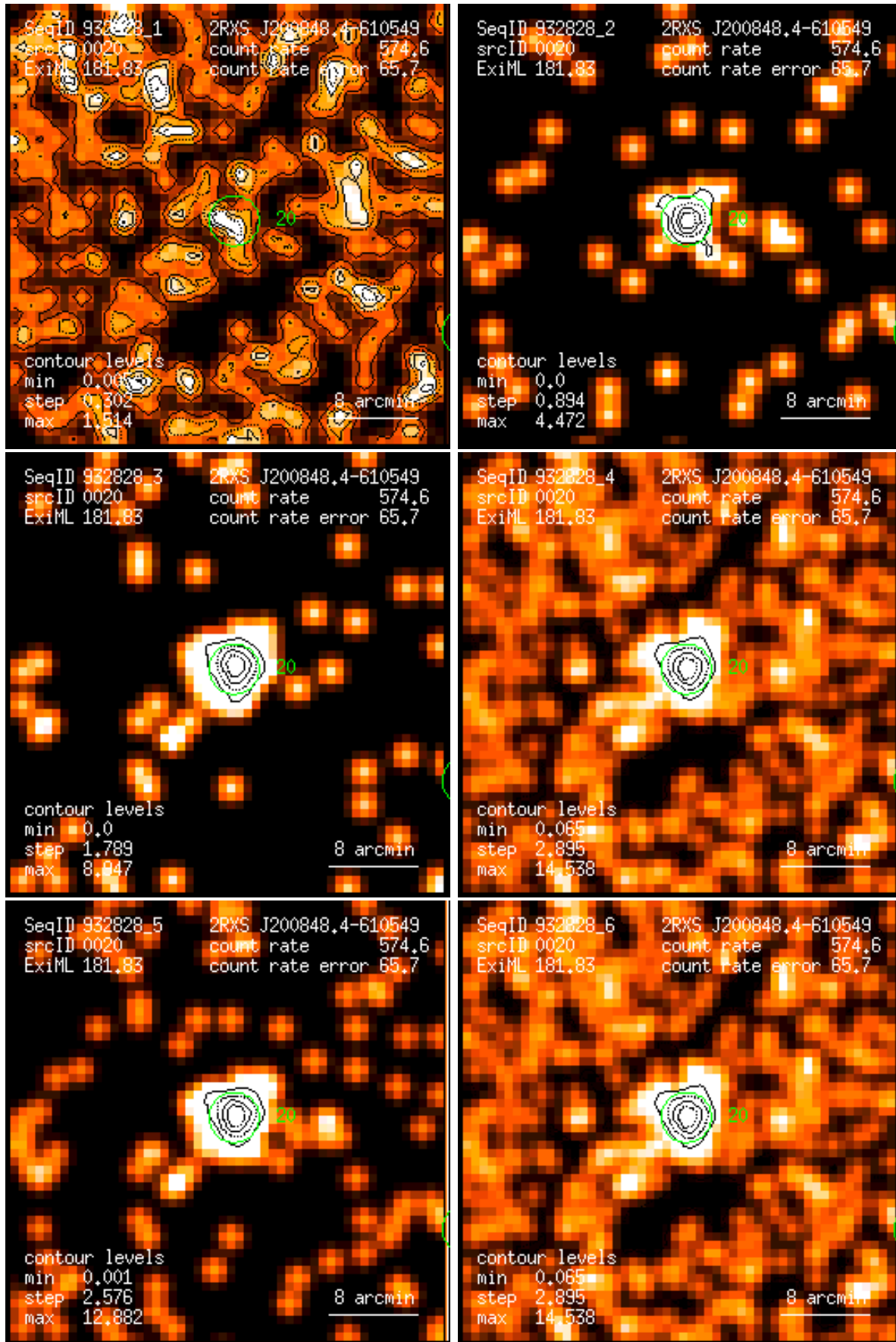
Figure 20: RASS 932828: detection 0020: band rate images, Gaussian filter: (1) PSPC channels 11 – 41, (2) 52 – 90, (3) 91 – 201, (4) 11 – 235, (5) 52 – 201, (6) 11 – 201. Broad band rates in counts/ks. Band rate contour levels in counts/ks/arcmin 2 .
