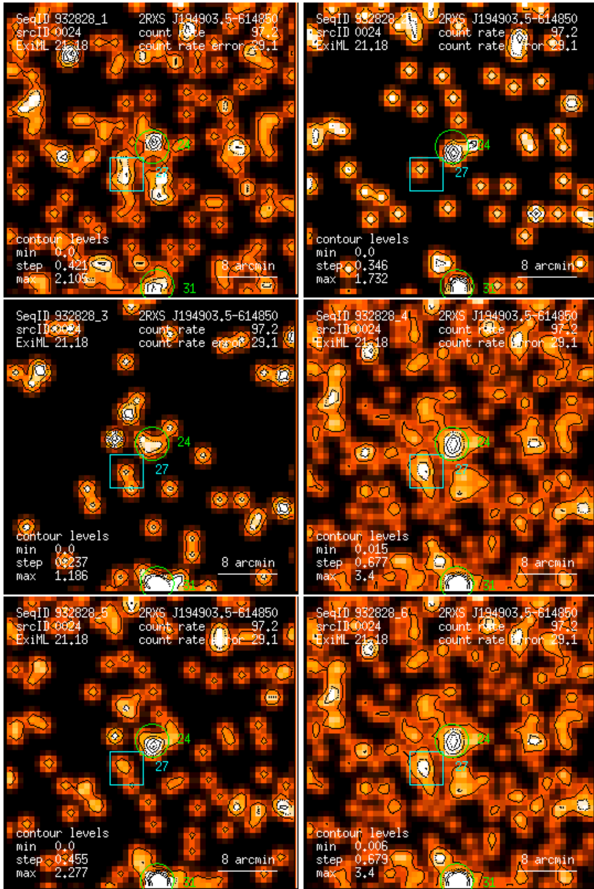
Figure 24: RASS 932828: detection 0024: band rate images, Gaussian filter: (1) PSPC channels 11 – 41, (2) 52 – 90, (3) 91 – 201, (4) 11 – 235, (5) 52 – 201, (6) 11 – 201. Broad band rates in counts/ks. Band rate contour levels in counts/ks/arcmin 2 .
