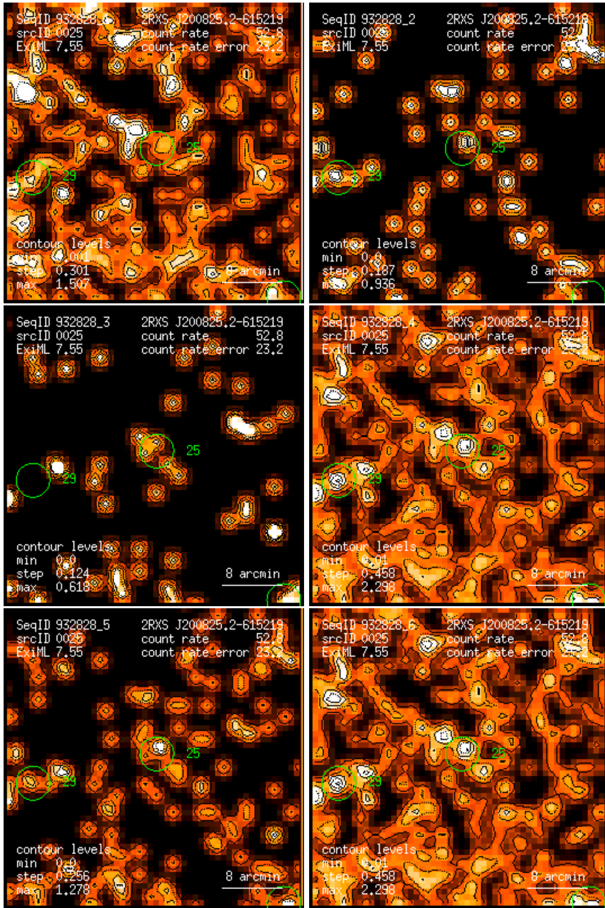
Figure 25: RASS 932828: detection 0025: band rate images, Gaussian filter: (1) PSPC channels 11 – 41, (2) 52 – 90, (3) 91 – 201, (4) 11 – 235, (5) 52 – 201, (6) 11 – 201. Broad band rates in counts/ks. Band rate contour levels in counts/ks/arcmin 2 .
