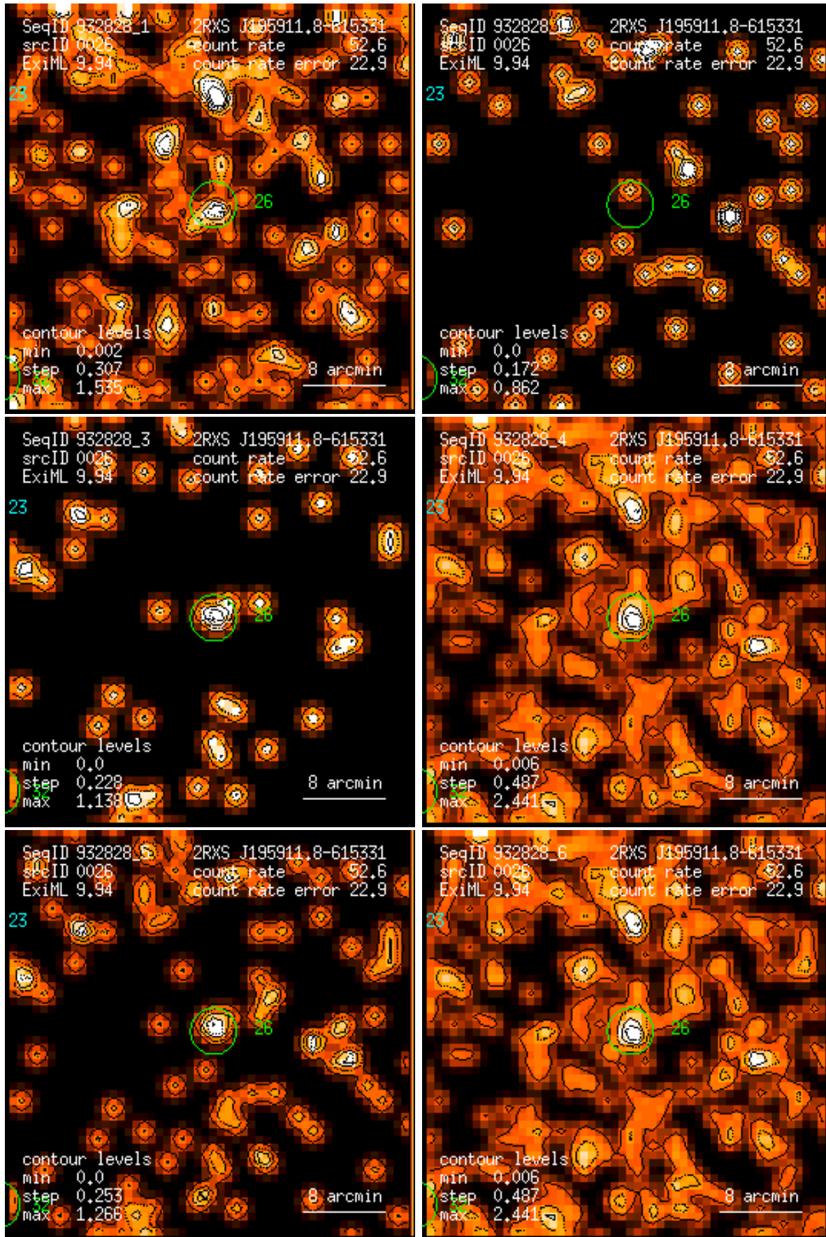
Figure 26: RASS 932828: detection 0026: band rate images, Gaussian filter: (1) PSPC channels 11 – 41, (2) 52 – 90, (3) 91 – 201, (4) 11 – 235, (5) 52 – 201, (6) 11 – 201. Broad band rates in counts/ks. Band rate contour levels in counts/ks/arcmin 2 .
