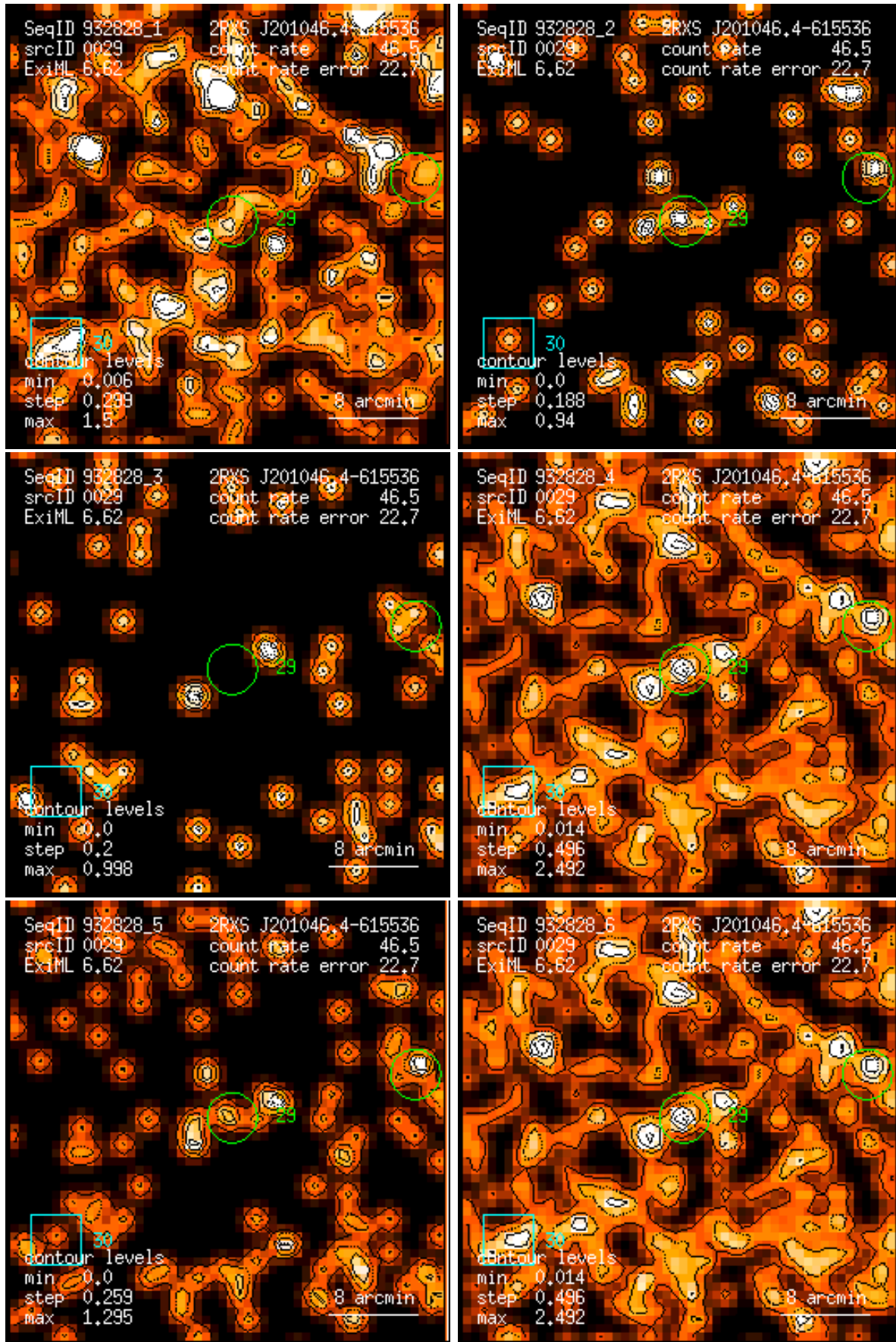
Figure 29: RASS 932828: detection 0029: band rate images, Gaussian filter: (1) PSPC channels 11 – 41, (2) 52 – 90, (3) 91 – 201, (4) 11 – 235, (5) 52 – 201, (6) 11 – 201. Broad band rates in counts/ks. Band rate contour levels in counts/ks/arcmin 2 .
