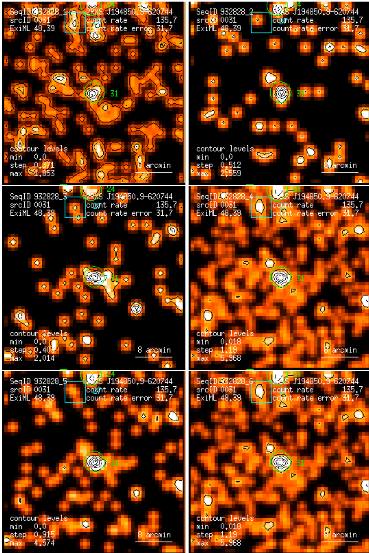
Figure 31: RASS 932828: detection 0031: band rate images, Gaussian filter: (1) PSPC channels 11 – 41, (2) 52 – 90, (3) 91 – 201, (4) 11 – 235, (5) 52 – 201, (6) 11 – 201. Broad band rates in counts/ks. Band rate contour levels in counts/ks/arcmin 2 .
