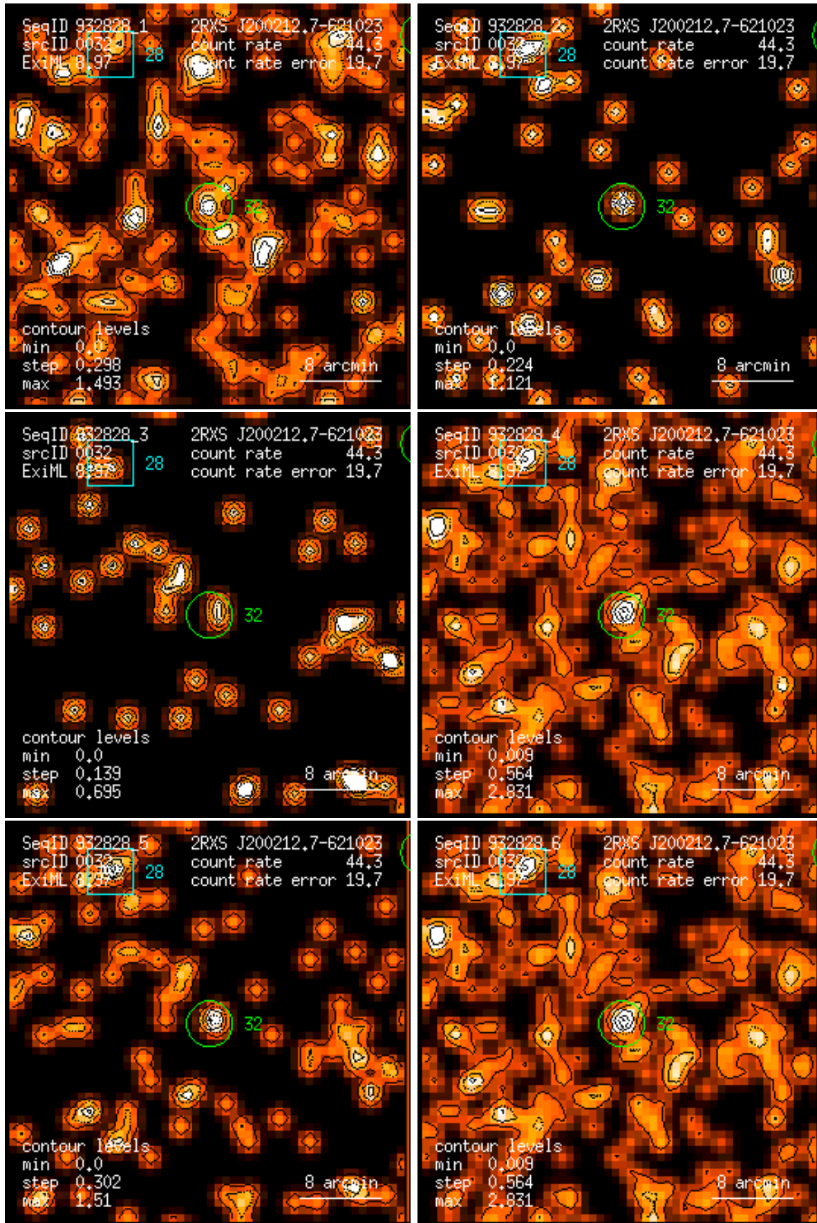
Figure 32: RASS 932828: detection 0032: band rate images, Gaussian filter: (1) PSPC channels 11 – 41, (2) 52 – 90, (3) 91 – 201, (4) 11 – 235, (5) 52 – 201, (6) 11 – 201. Broad band rates in counts/ks. Band rate contour levels in counts/ks/arcmin 2 .
