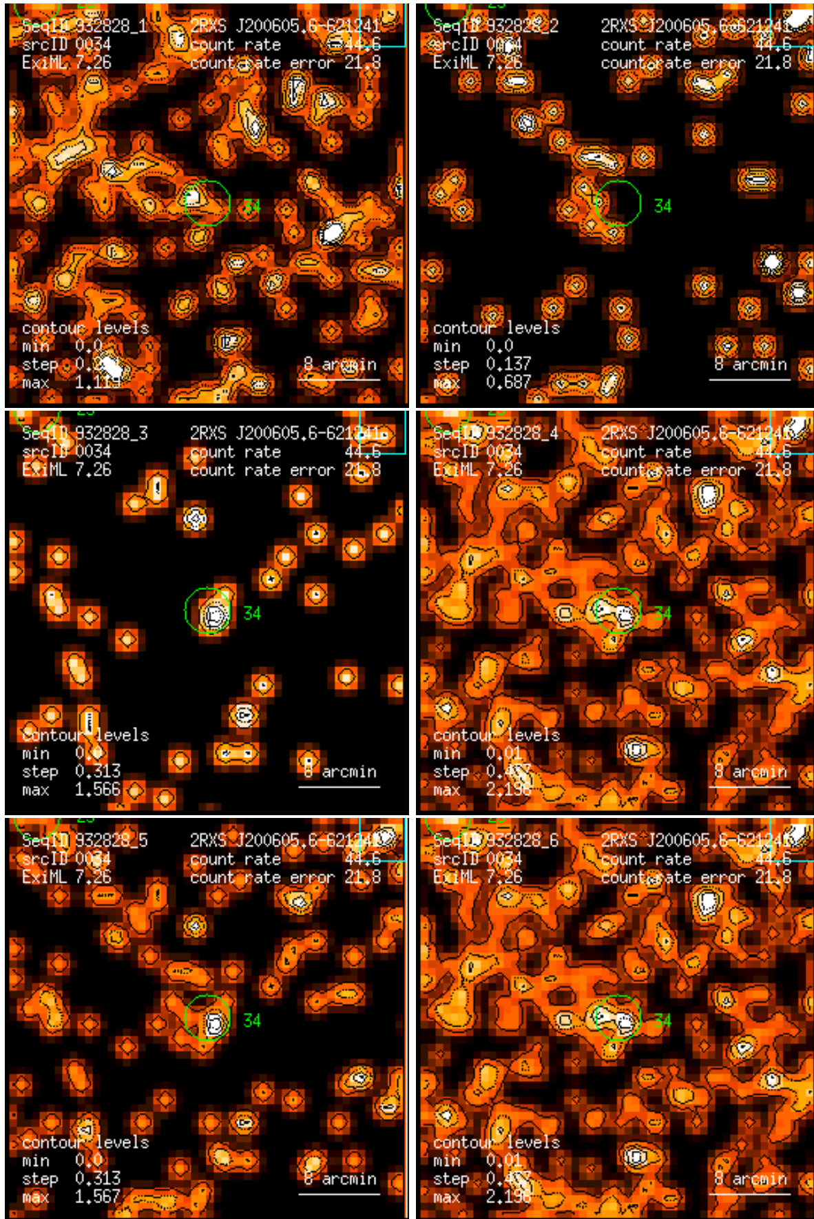
Figure 34: RASS 932828: detection 0034: band rate images, Gaussian filter: (1) PSPC channels 11 – 41, (2) 52 – 90, (3) 91 – 201, (4) 11 – 235, (5) 52 – 201, (6) 11 – 201. Broad band rates in counts/ks. Band rate contour levels in counts/ks/arcmin 2 .
